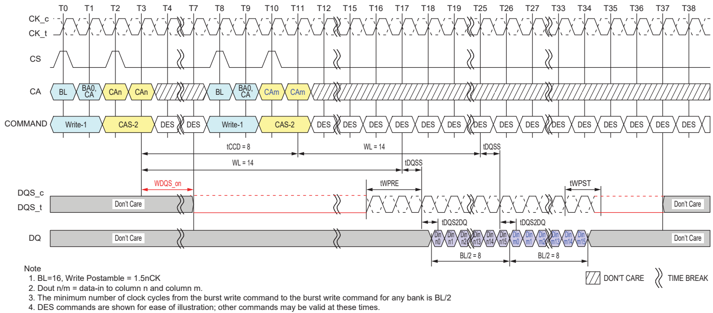
Figure 4.34 — Seamless Writes Operation: t_{CCD} = \text{Min}, 1.5n\text{CK} Postamble
