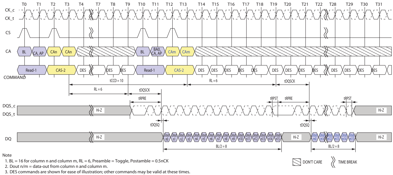
Figure 4.25 — Consecutive Reads Operation: t_{CCD} = \text{Min} + 2 , Preamble = Toggle, 0.5nCK Postamble
