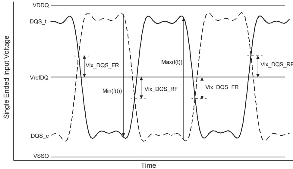
Figure 7.13 — Vix Definition (DQS)
