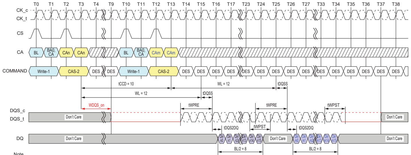
Figure 4.38 — Consecutive Writes Operation: tCCD = Min + 2, 1.5nCK Postamble
