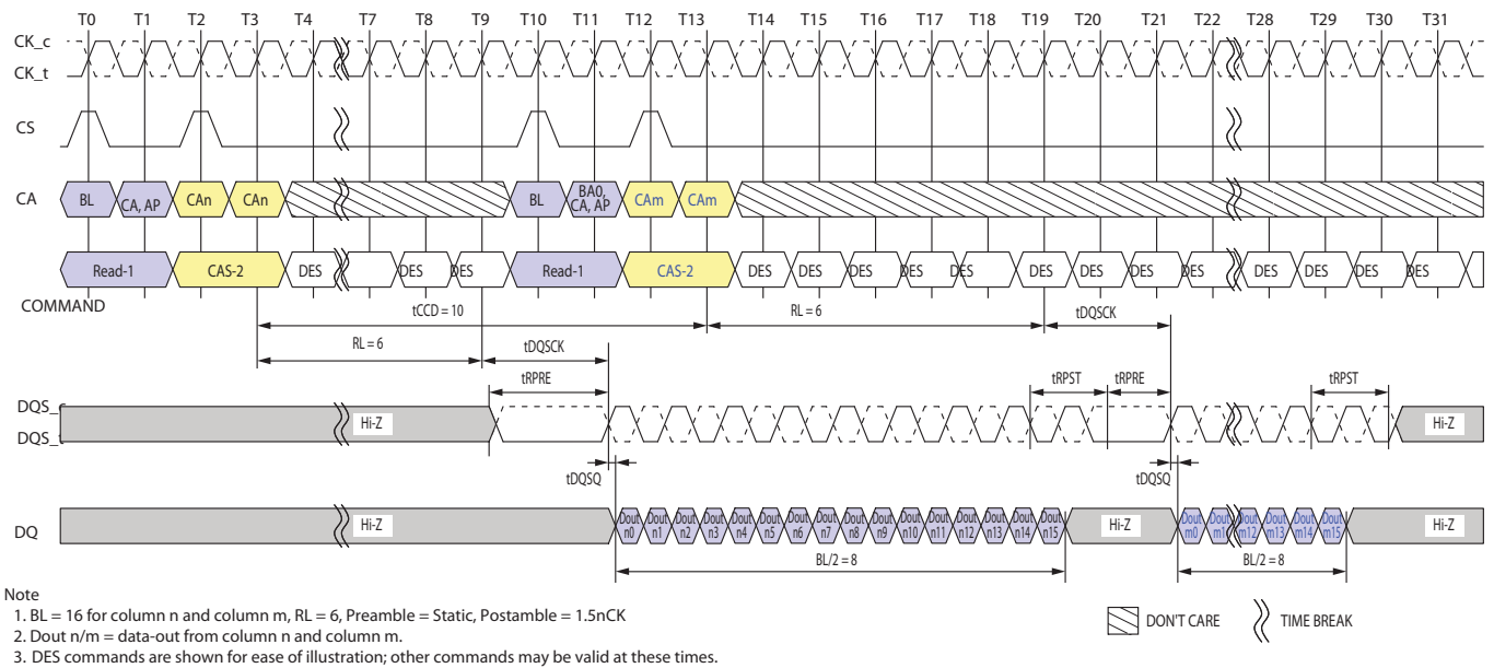
Figure 4.26 — Consecutive Reads Operation: t_{CCD} = \text{Min} + 2 , Preamble = Static, 1.5nCK Postamble
