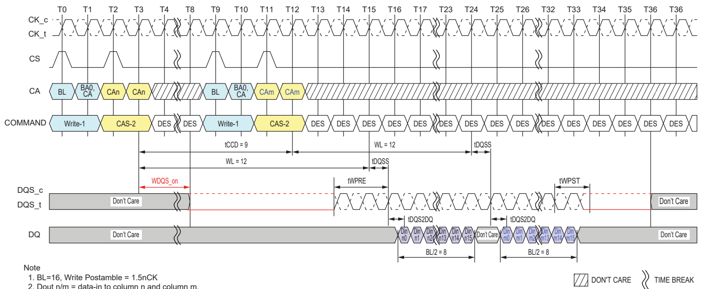
Figure 4.36 — Consecutive Writes Operation: t_{CCD} = Min + 1, 1.5nCK Postamble
