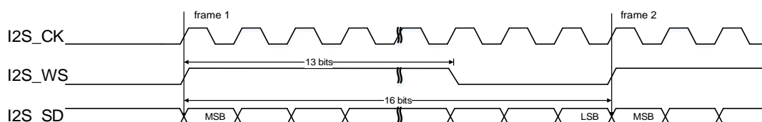
Figure 18-40. PCM standard long frame synchronization mode timing diagram (DTLEN=00, CHLEN=0, CKPL=0)
