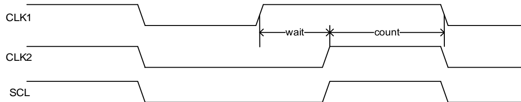
Figure 17-4. Clock synchronization
