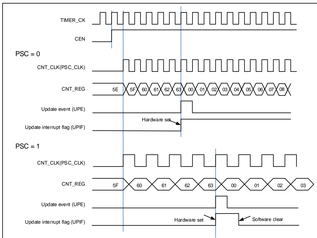
Figure 15-4. Timing chart of up counting mode, PSC=0/1
