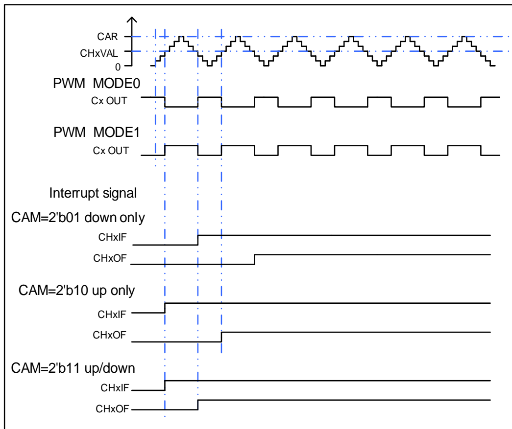
Figure 15-45. CAPWM timechart
