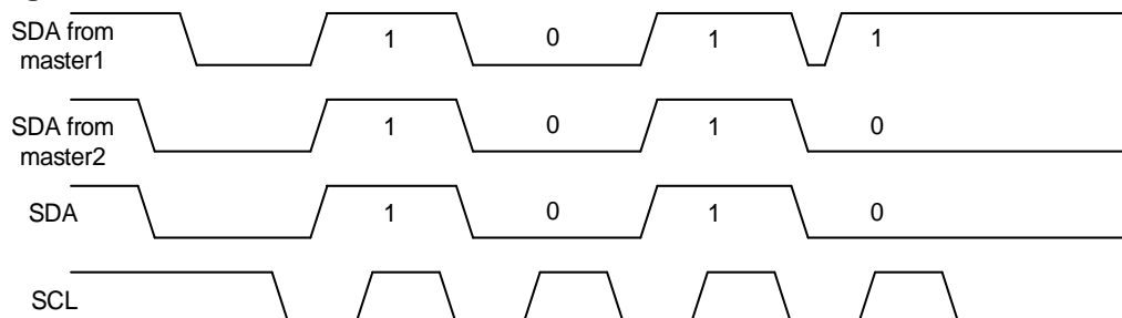
Figure 17-5. SDA Line arbitration
