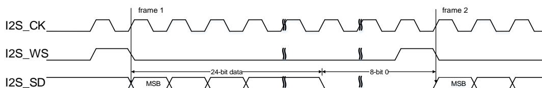
Figure 18-36. PCM standard short frame synchronization mode timing diagram (DTLEN=01, CHLEN=1, CKPL=0)
