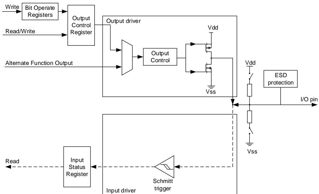
Figure 7.3. Output configuration
