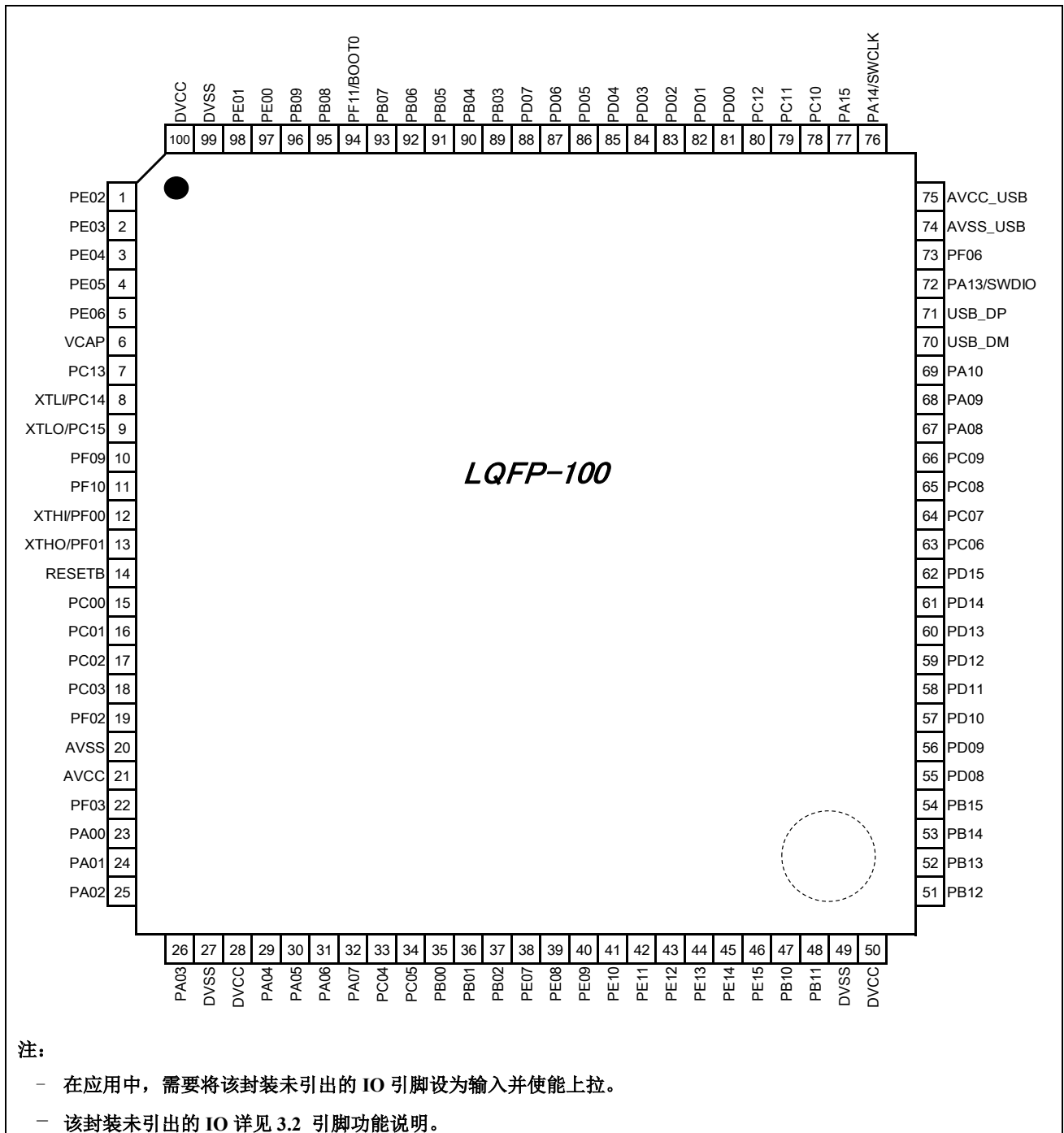
HC32L072PATA-LQFP100
