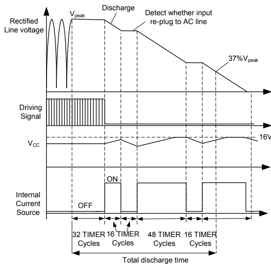
Figure 10: X-Cap Discharger
