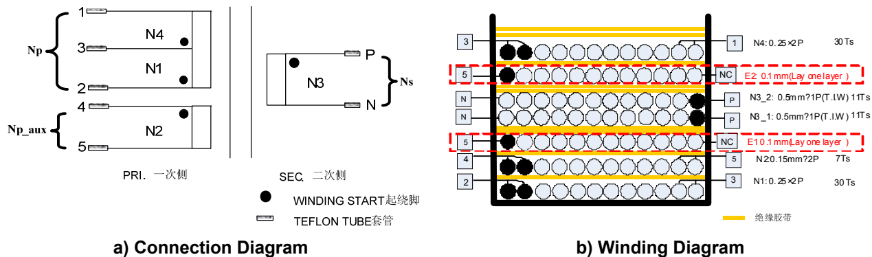
Figure18: Transformer Structure
