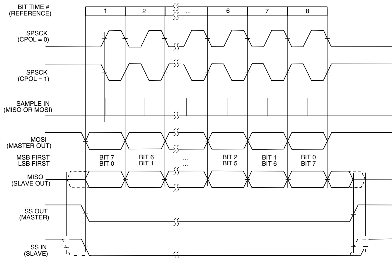
Figure 35-38. SPI clock formats ( CPHA = 0 )
