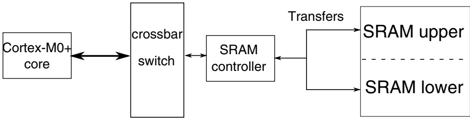
Figure 3-19. SRAM configuration
