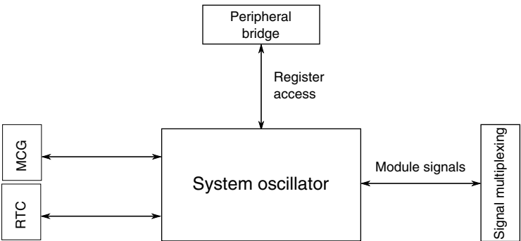
Figure 3-15. OSC configuration
