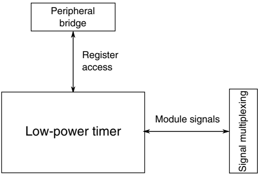
Figure 3-26. LPT configuration
