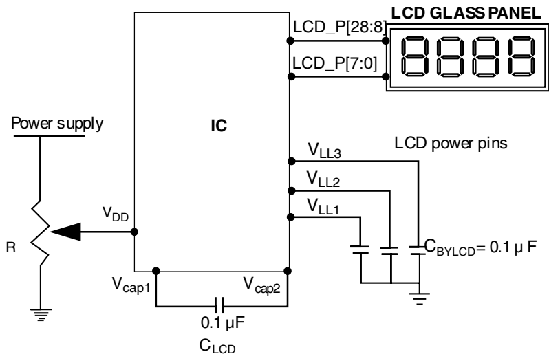
Figure 40-43. Power connections for contrast control
