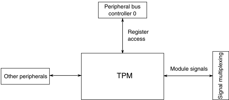
Figure 3-24. TPM configuration
