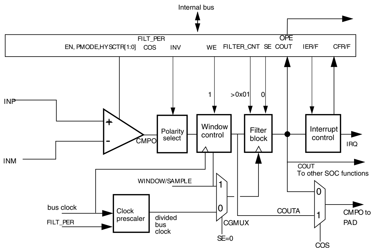
Figure 29-23. Windowed/Filtered mode
