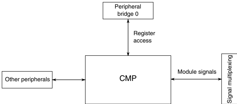
Figure 3-23. CMP configuration
