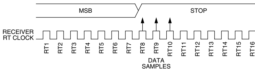
Figure 38-31. Slow data
