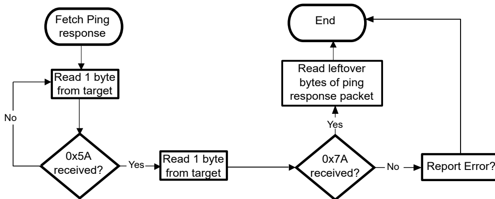
Figure 123. Host reads ping response from target via FCAN
