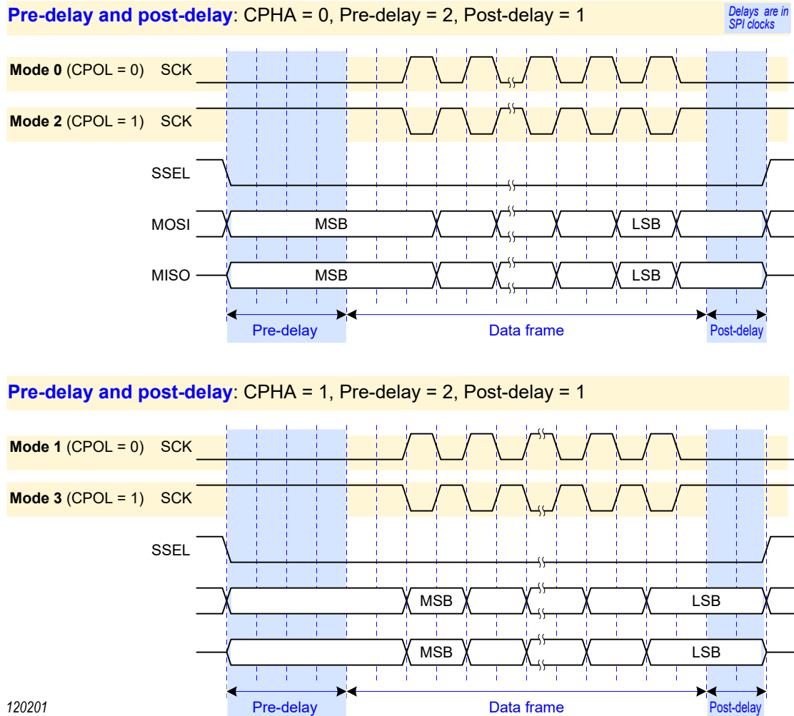
Figure 167. Pre-delay and post-delay
