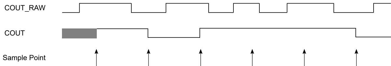
Figure 276. Sampled, Non-Filtered mode timing diagram
