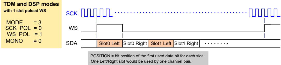
Figure 180. TDM and DSP modes with 1 slot pulsed WS
