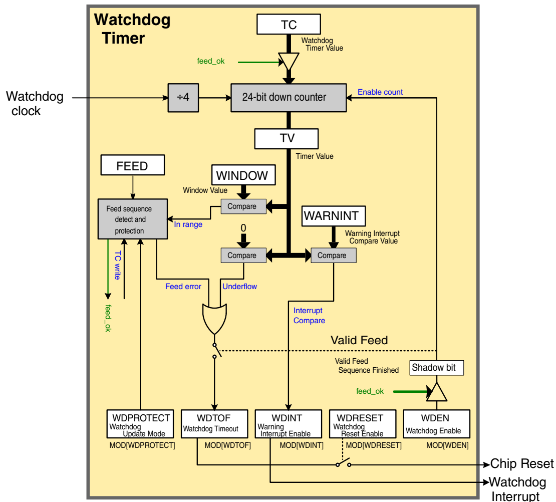
Figure 150. Windowed Watchdog Timer block diagram
