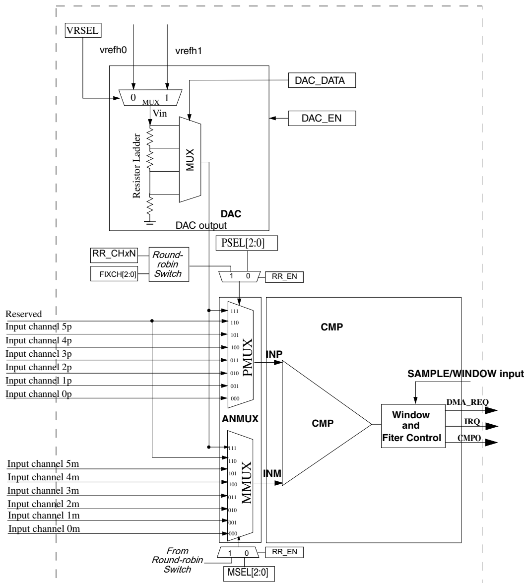
Figure 271. Block Diagram
