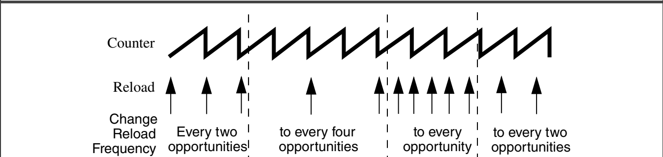
Figure 236. Full and half cycle reload frequency change
