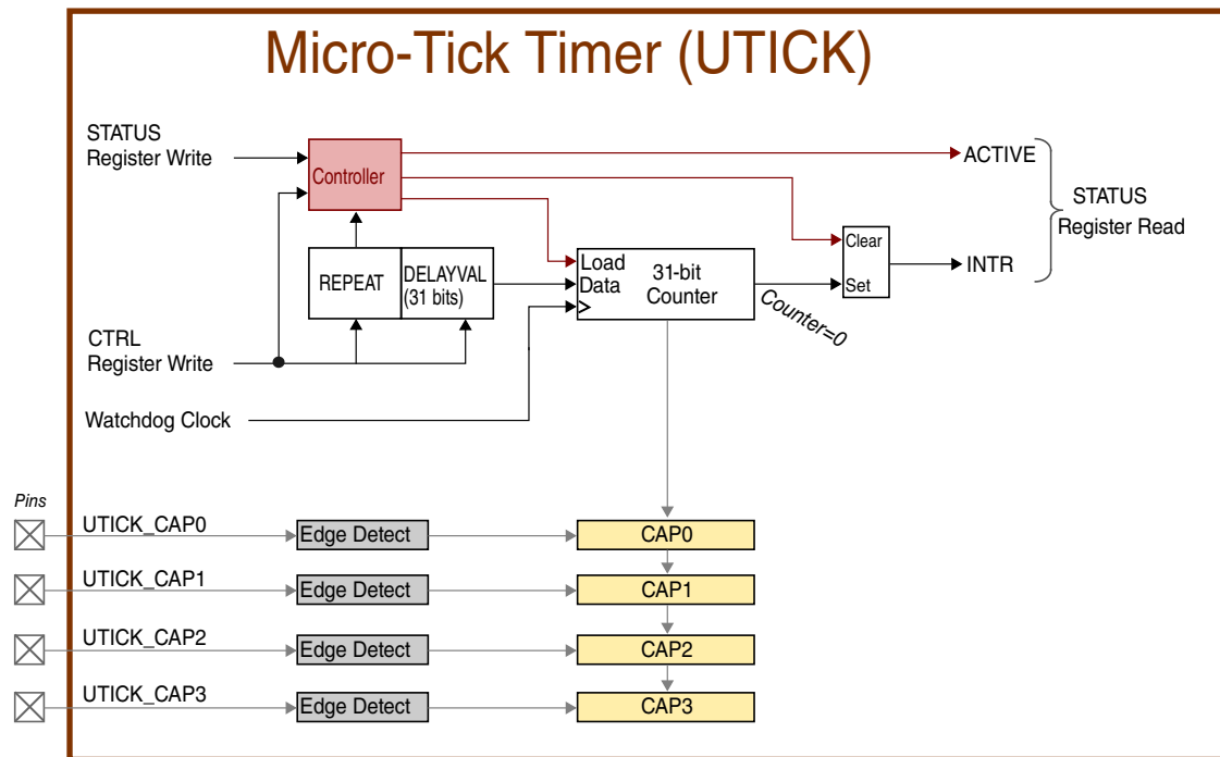
Figure 149. UTICK block diagram
