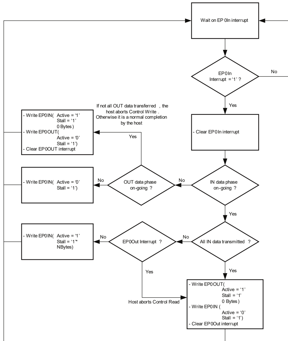
Figure 161. Flowchart of control endpoint 0 - IN
