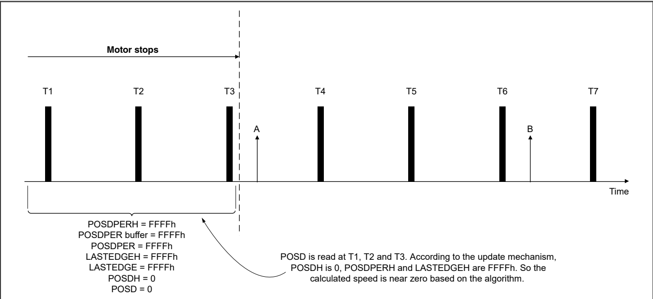
Figure 245. Speed measurement at time point T1~T3
