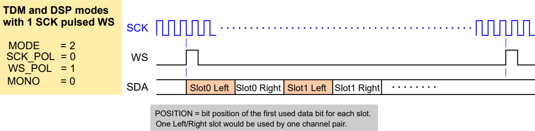
Figure 179. TDM and DSP modes with 1 SCK pulsed WS
