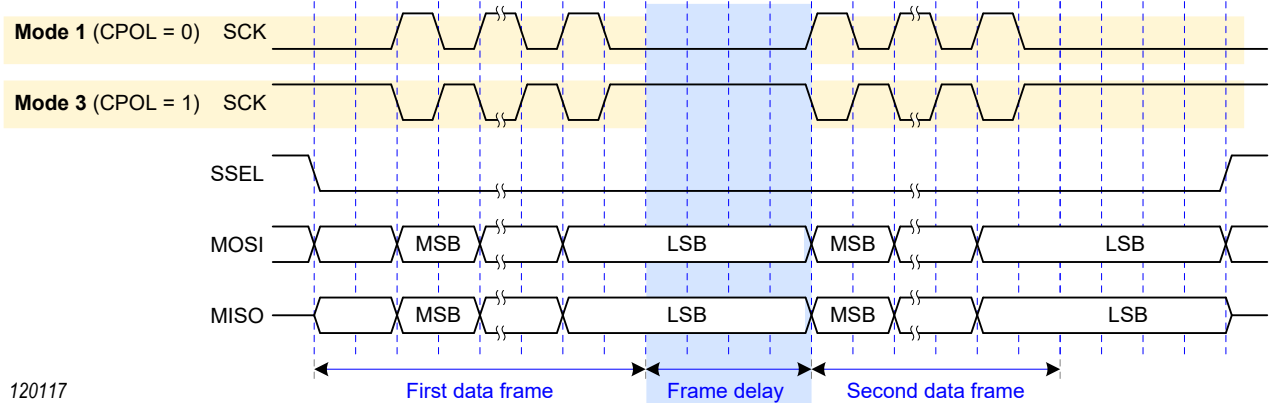
Figure 168. Frame delay
