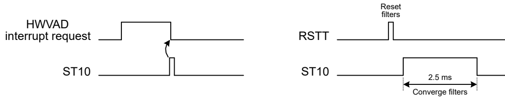
Figure 259. Use of ST10 and RSTT controls (in the HWVADST10 and HWVADRSTT registers)
