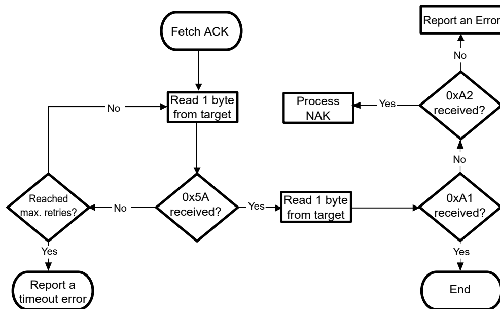
Figure 124. Host reads ACK packet from target via CAN
