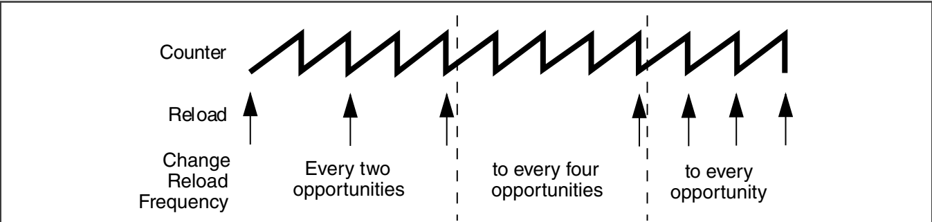
Figure 234. Full cycle reload frequency change
