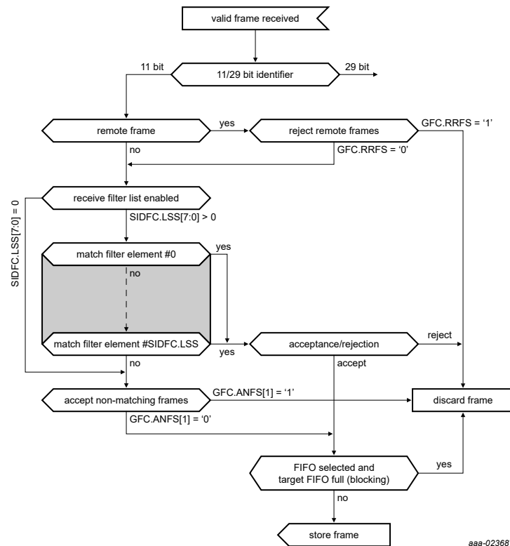
Figure 191. Standard message ID filter path
