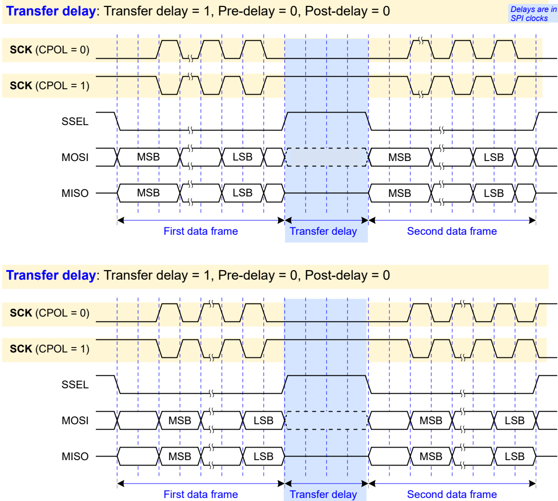
Figure 169. Transfer delay
