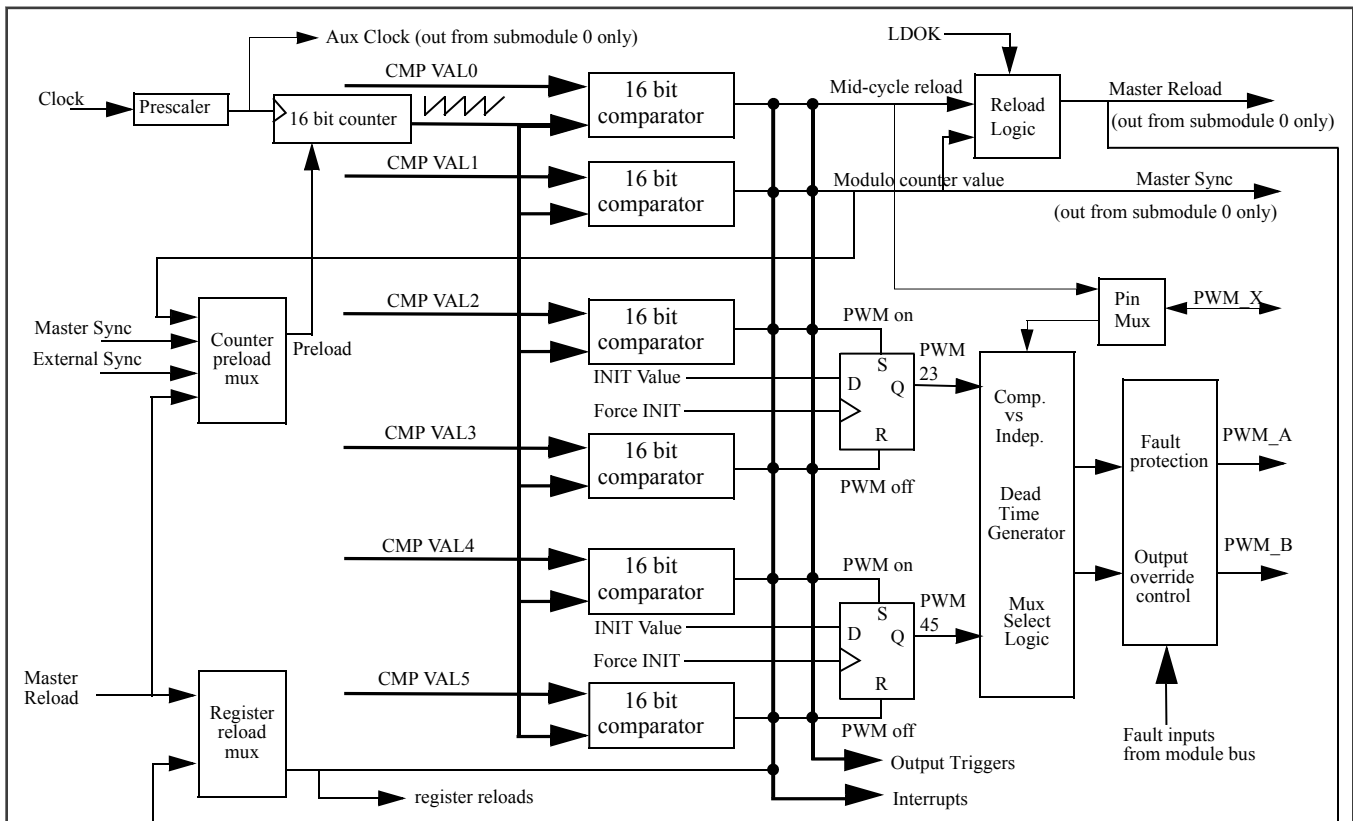
Figure 204. PWM submodule block diagram
