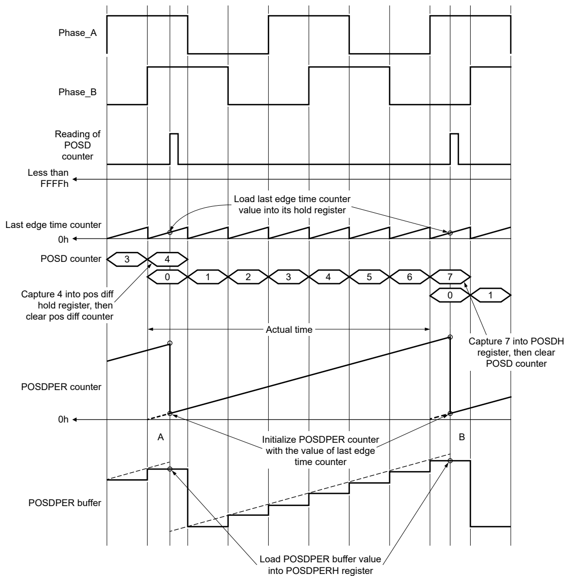
Figure 242. Counters behavior and updating mechanism
