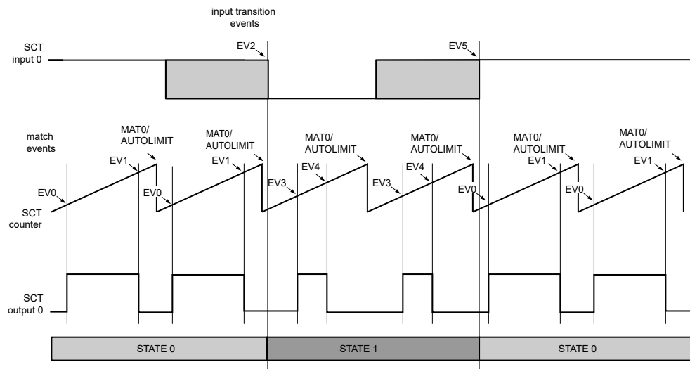
Figure 141. SCT configuration example
