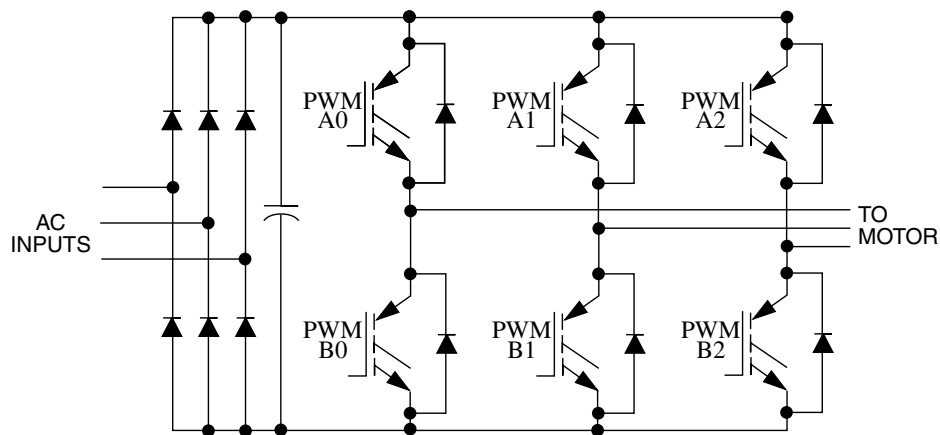
Figure 221. Typical 3 phase AC motor drive
