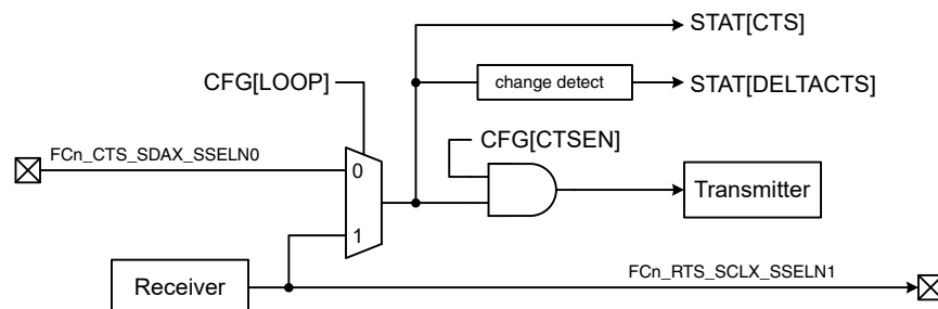
Figure 164. Hardware flow control using RTS and CTS
