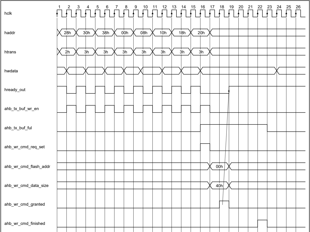
Figure 52. AHB write access (WRAP8, 64-bit, bufferable)
