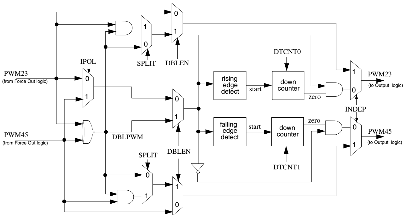
Figure 222. Deadtime Insertion Logic for each submodule
