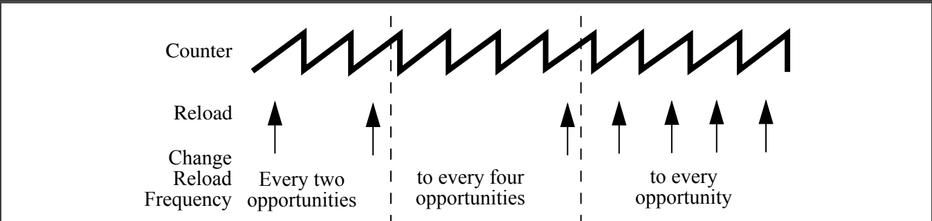
Figure 235. Half cycle reload frequency change
