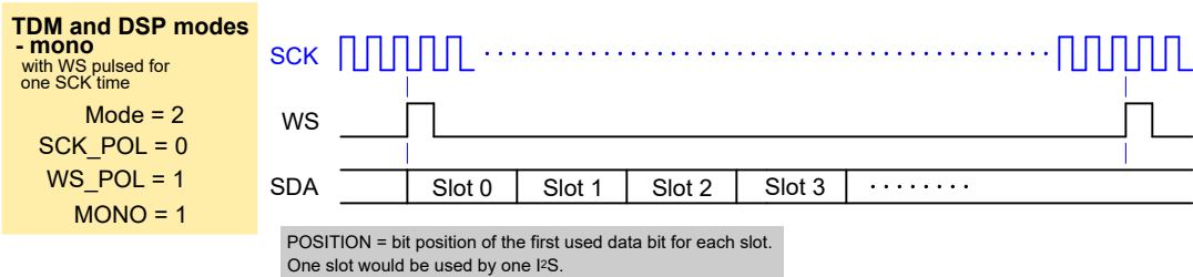
Figure 183. TDM and DSP modes, mono, with WS pulsed for one SCK time
