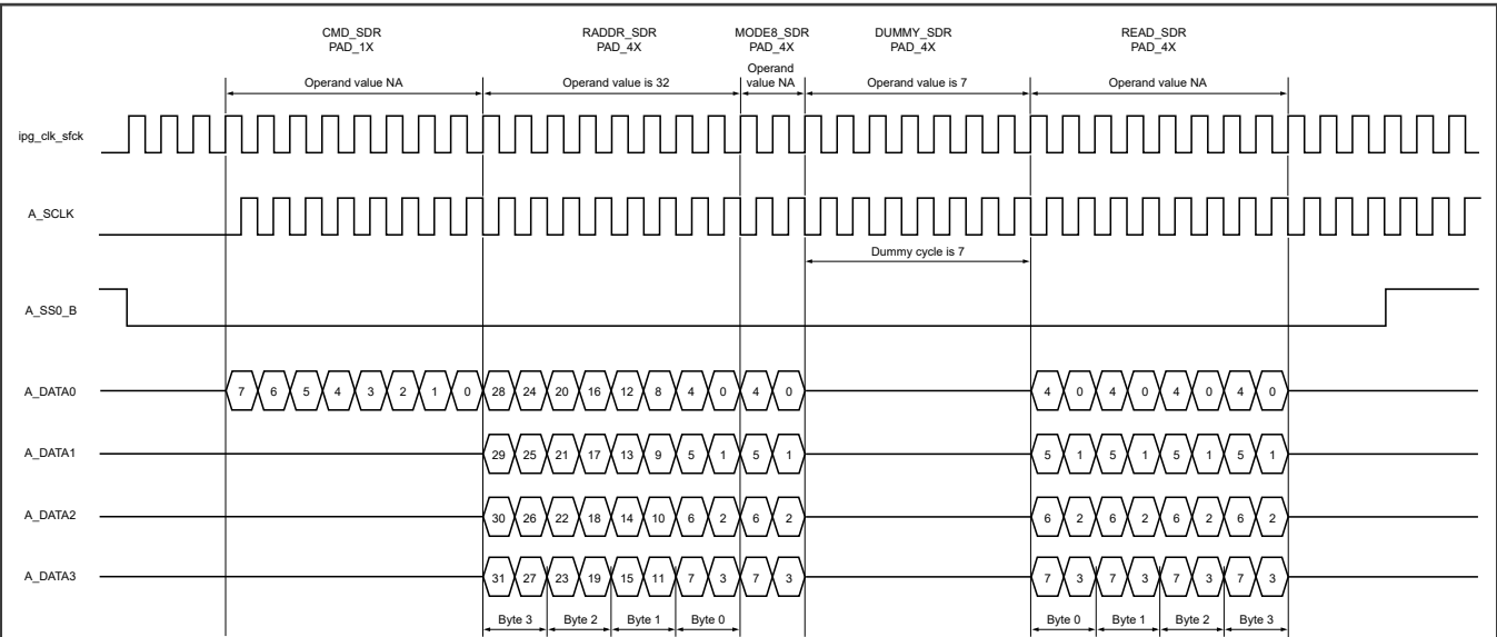
Figure 40. Flash memory access sequence example (SDR quad I/O read sequence)
