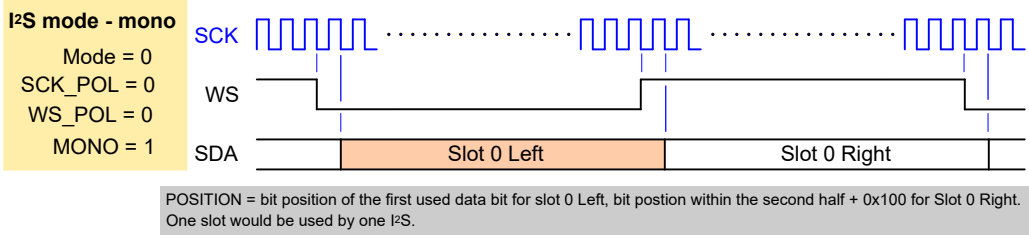
Figure 181. I 2 S mode, mono
