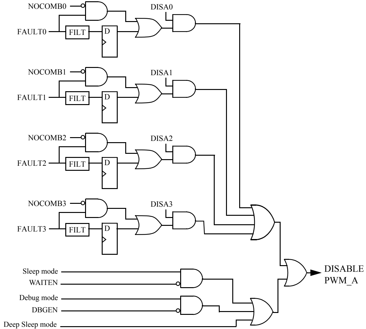
Figure 230. Fault decoder for PWM_A
