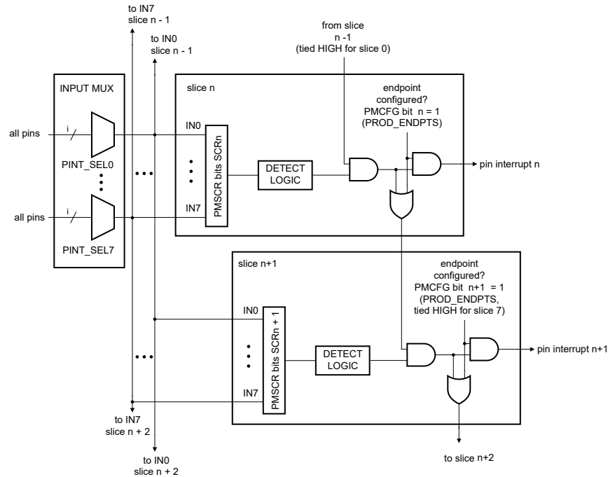
Figure 80. Pattern match engine connections
