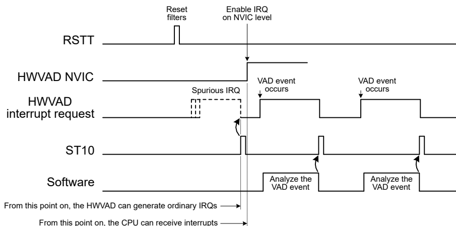
Figure 260. Complete HWVAD setup
