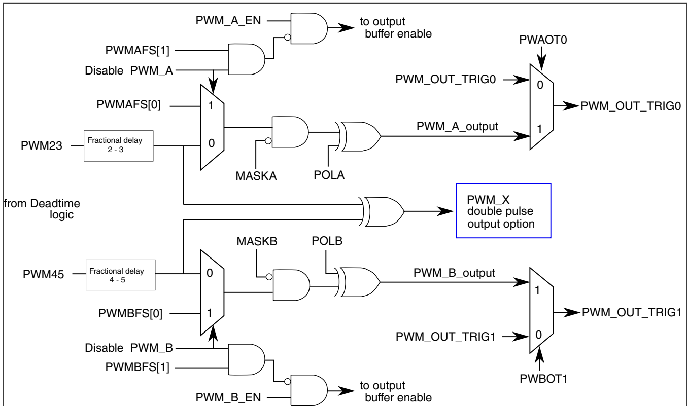
Figure 227. Output logic for each submodule
