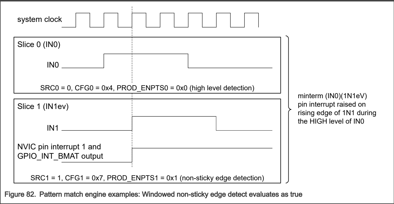
Figure 81. Pattern match engine examples: sticky edge detect
