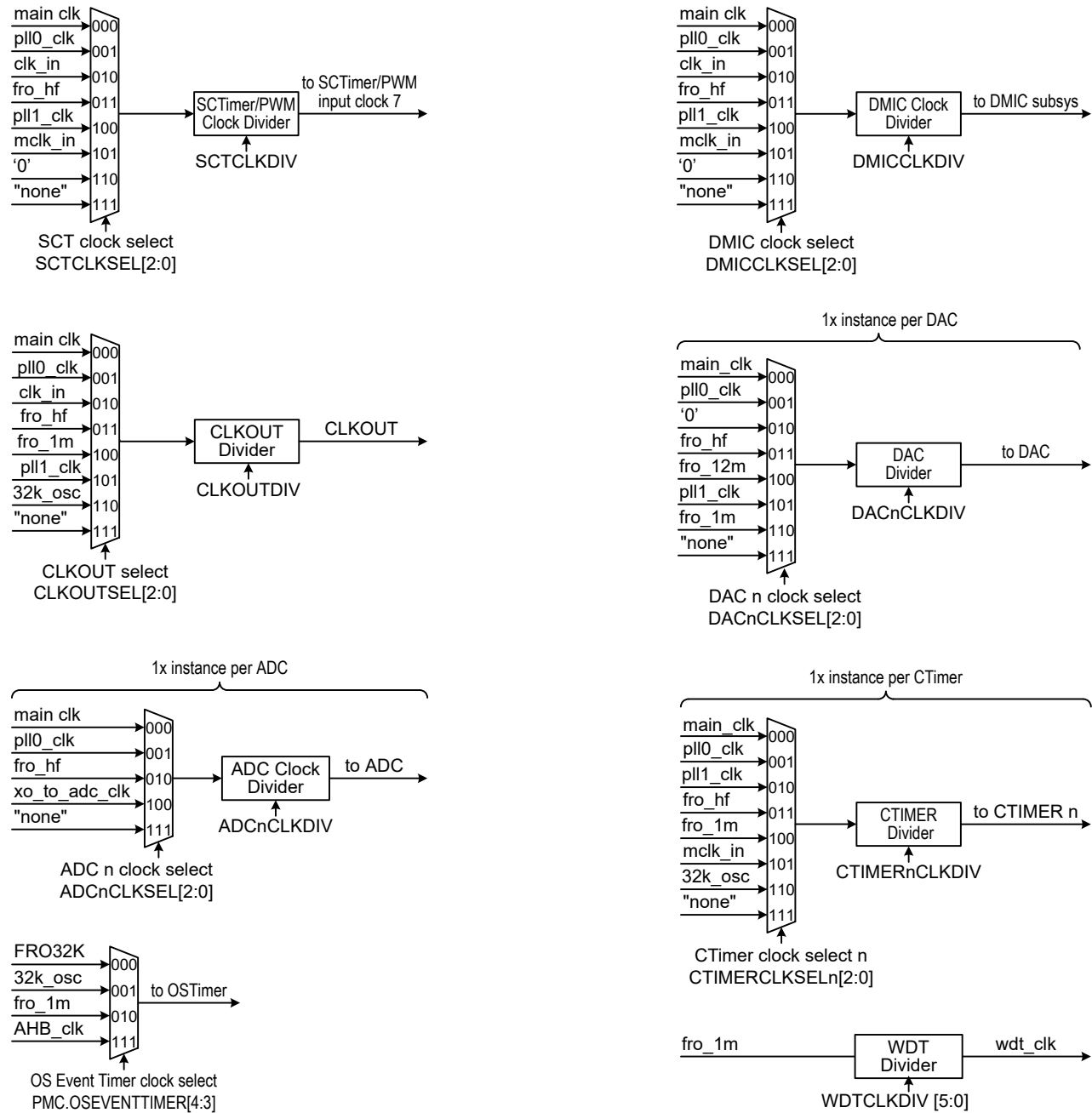
Figure 11. Clock generation (Part 3 of 3)
