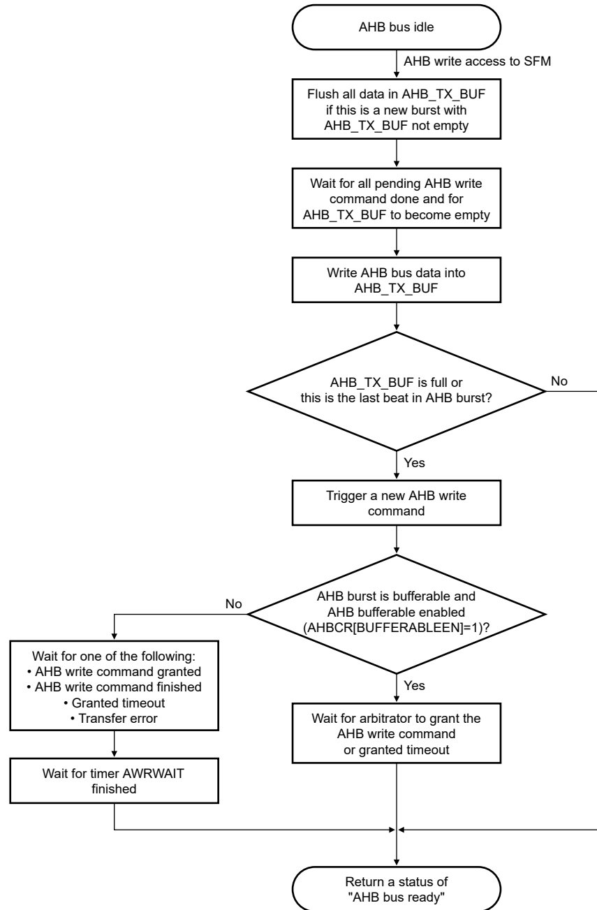
Figure 50. Hardware operation in response to AHB write access to flash memory
