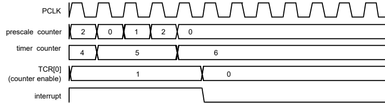
Figure 137. A timer cycle in which PR=2, MRx=6, and both interrupt and reset on match are enabled
