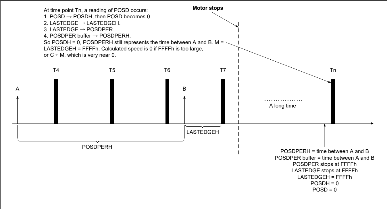
Figure 250. Speed measurement at time point Tn
