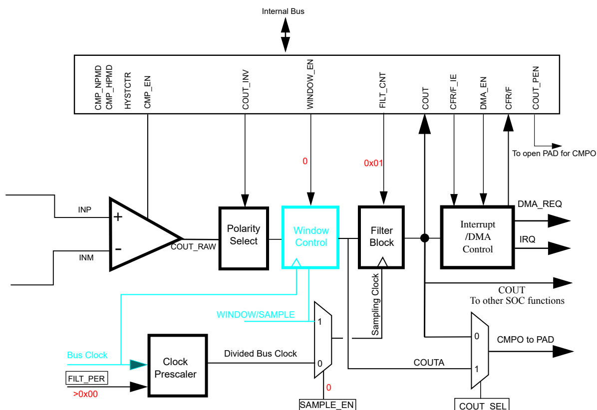
Figure 275. Sampled, Non-Filtered (#3B): sampling interval internally derived
