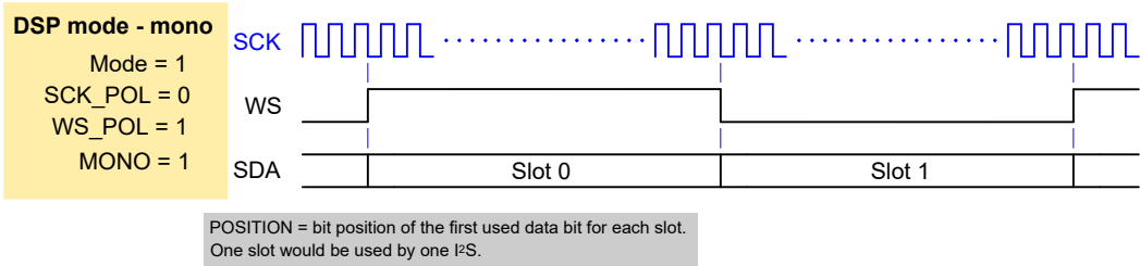
Figure 182. DSP mode, mono
