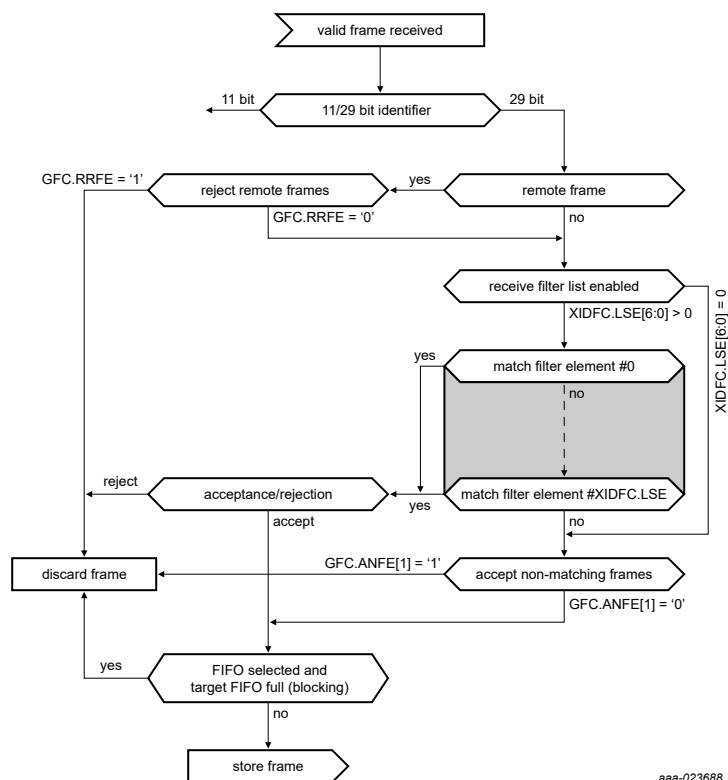
Figure 192. Extended message ID filter path
