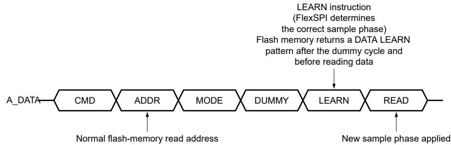
Figure 70. Data learning flow with flash-memory-provided preamble bit
