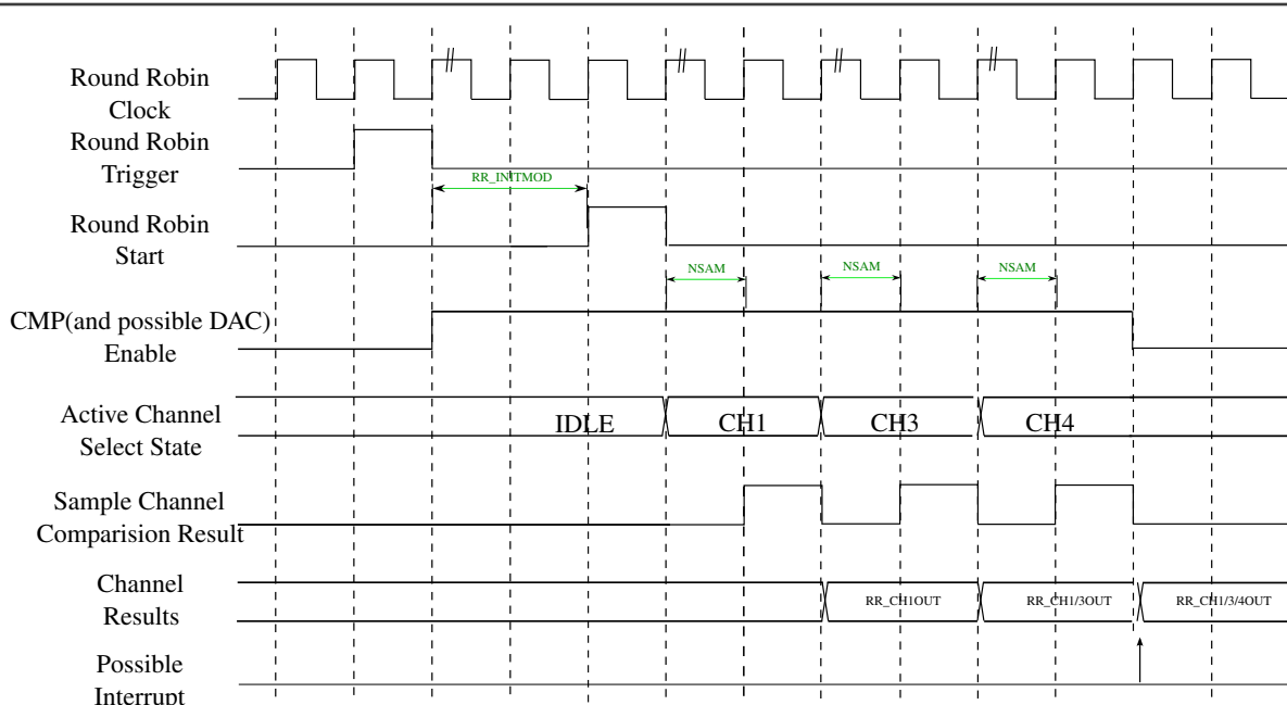
Figure 288. Trigger Mode
