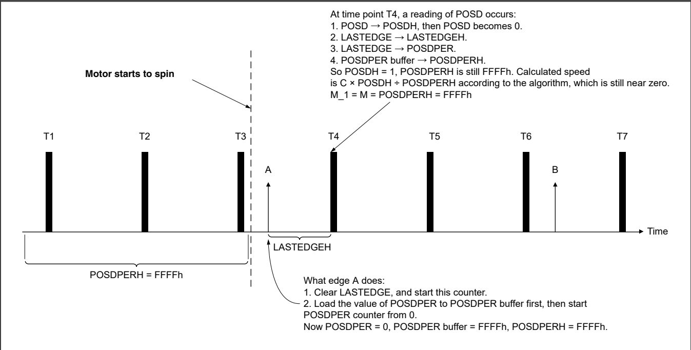
Figure 246. Speed measurement at time point T4
