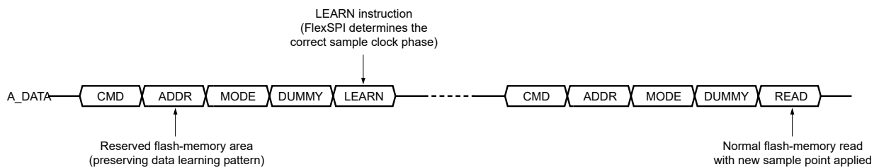
Figure 71. Data learning flow without flash-memory-provided preamble bit
