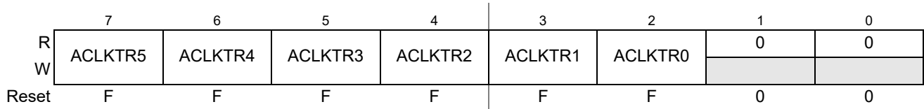
Figure 8-26. Autonomous Clock Trimming Register (CPMUACLKTR)
