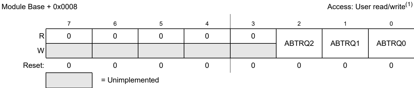
Figure 13-12. MSCAN Transmitter Message Abort Request Register (CANTARQ)
