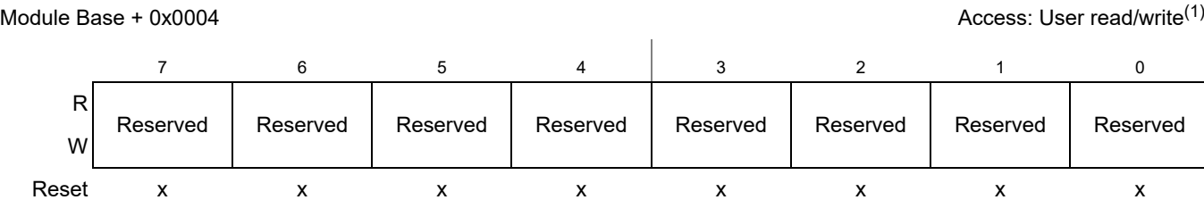
Figure 21-6. Reserved Register
