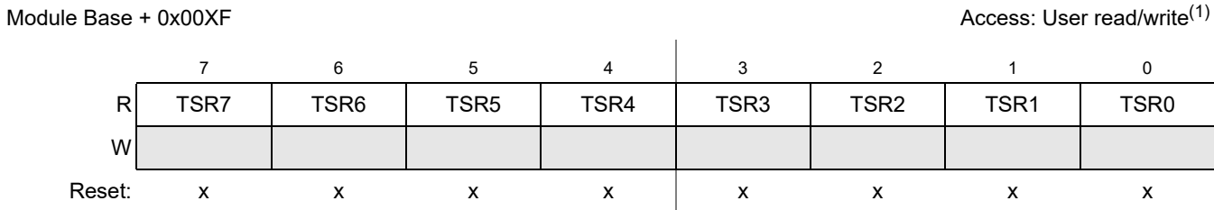
Figure 13-38. Time Stamp Register — Low Byte (TSRL)
