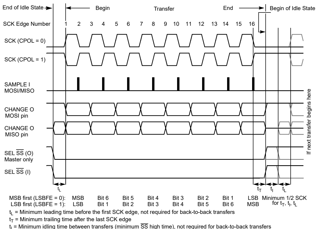
Figure 17-14. SPI Clock Format 1 (CPHA = 1), with 8-Bit Transfer Width selected (XFRW = 0)
