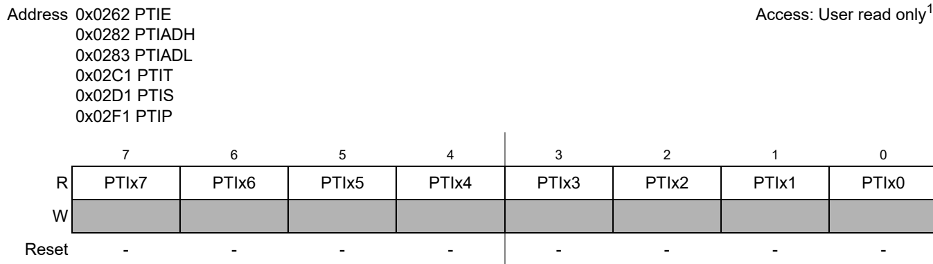
Figure 2-13. Port Input Register
