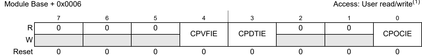
Figure 21-8. CAN Physical Layer Interrupt Enable Register (CPIE)
