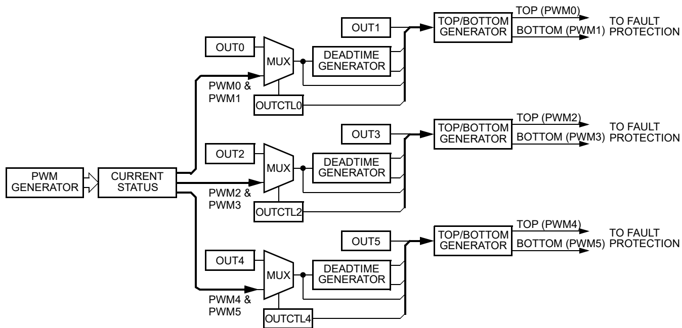
Figure 15-50. Deadtime Generators
