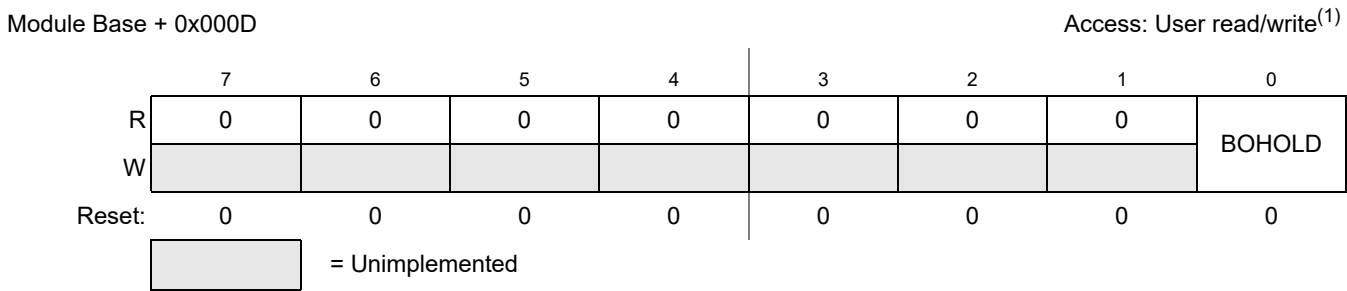
Figure 13-17. MSCAN Miscellaneous Register (CANMISC)
