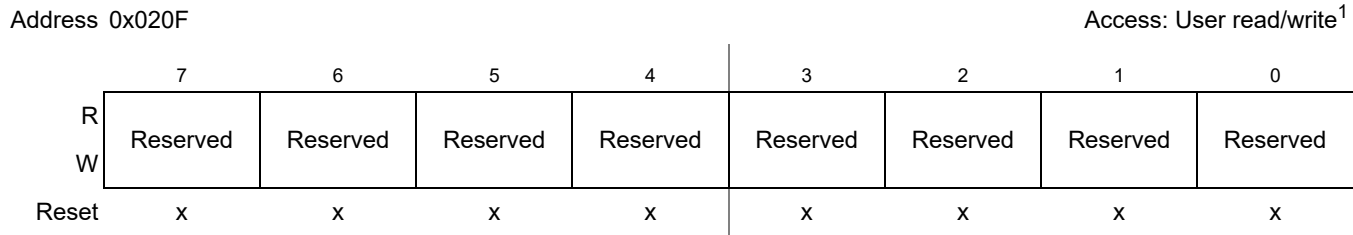
Figure 2-11. Reserved Register
