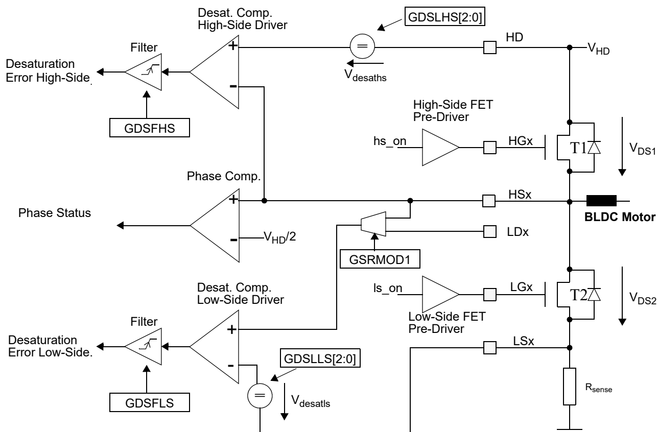
Figure 18-23. Desaturation Comparators and Phase Comparators in BLDC Mode (LDx not connected) 1
