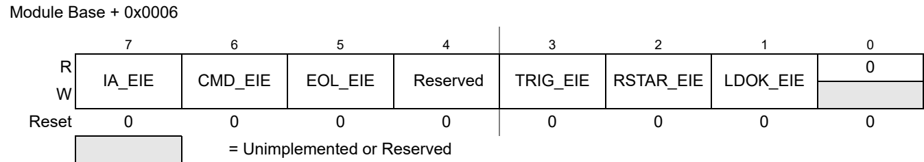
Figure 9-10. ADC Error Interrupt Enable Register (ADCEIE)
