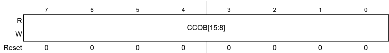
Figure 20-24. Flash Common Command Object 3 High Register (FCCOB3HI)
