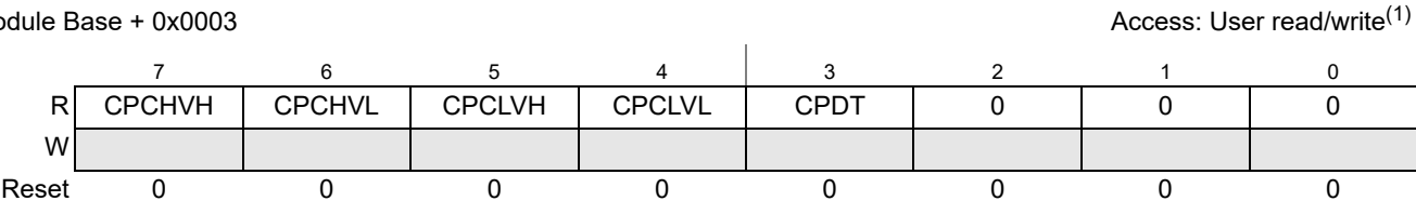
Figure 21-5. CAN Physical Layer Status Register (CPSR)
