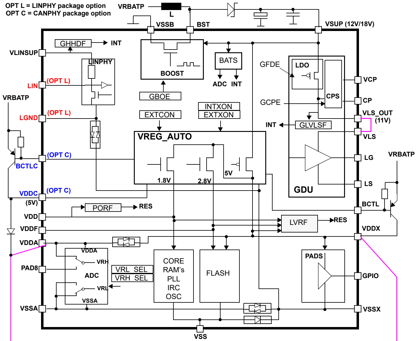
Figure 1-18. Power Domain Overview
