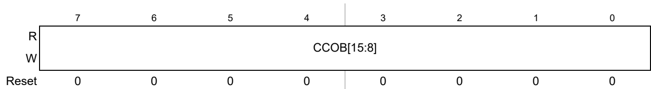
Figure 20-26. Flash Common Command Object 4 High Register (FCCOB4HI)
