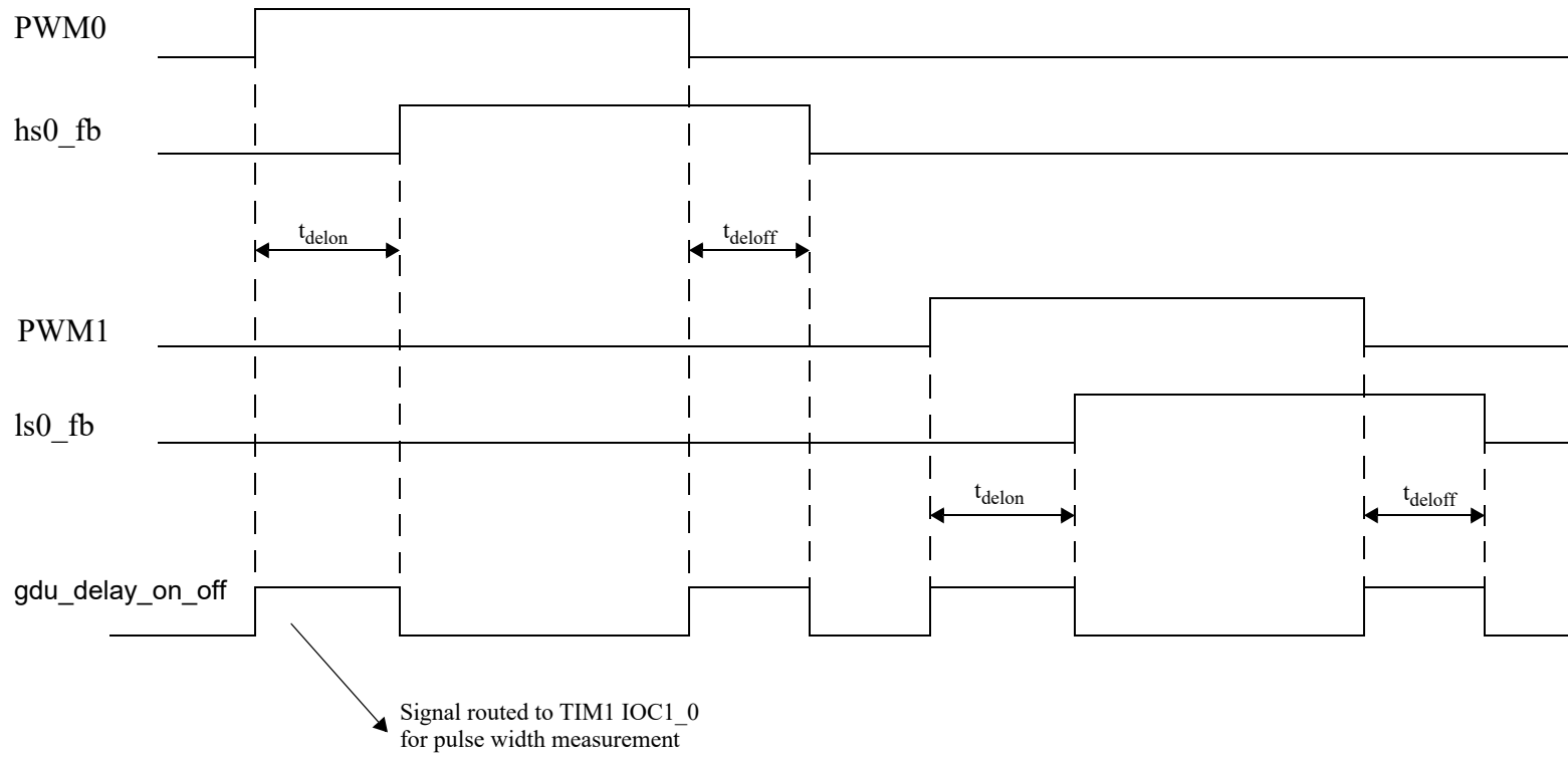
Figure 18-32. Measurement of GDU t_{\text{delon}} and t_{\text{deloff}}
