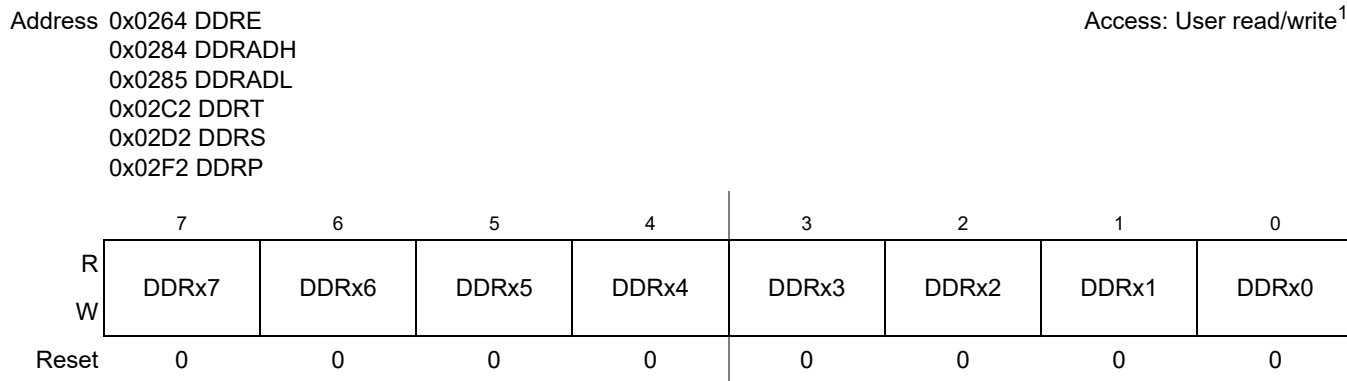
Figure 2-14. Data Direction Register
