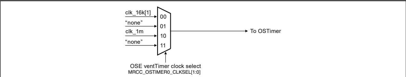
Figure 62. OSTimer clock
