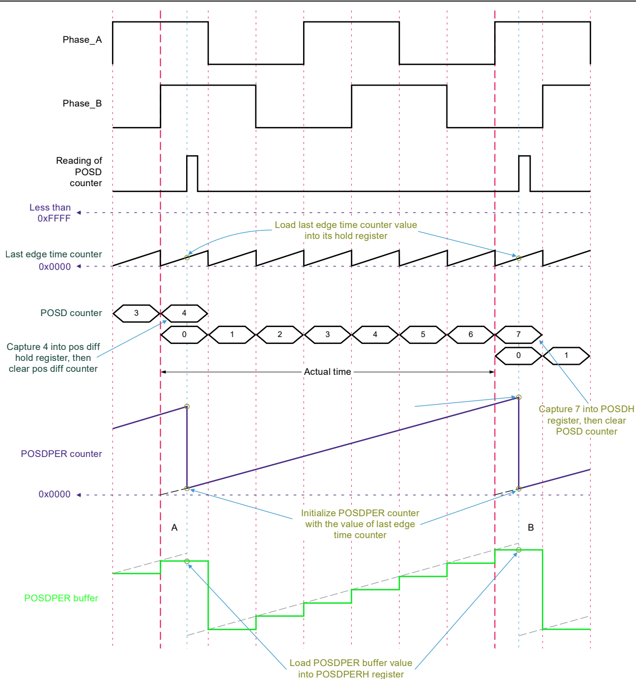
Figure 133. Counters behavior and updating mechanism
