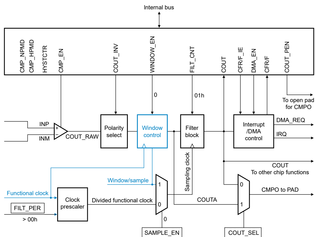
Figure 173. Sampled, Non-Filtered (#3B): sampling interval internally derived
