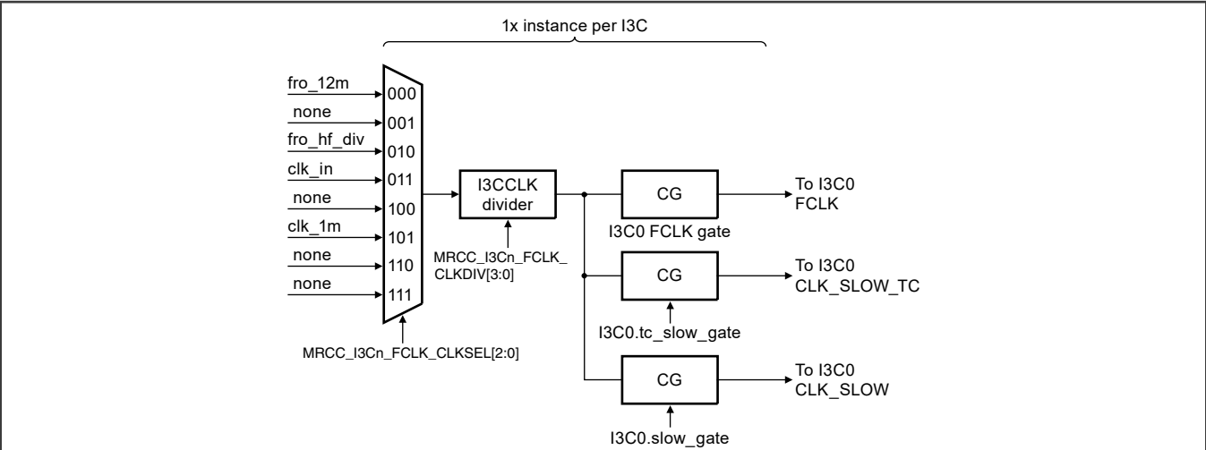
Figure 56. I3C clock
