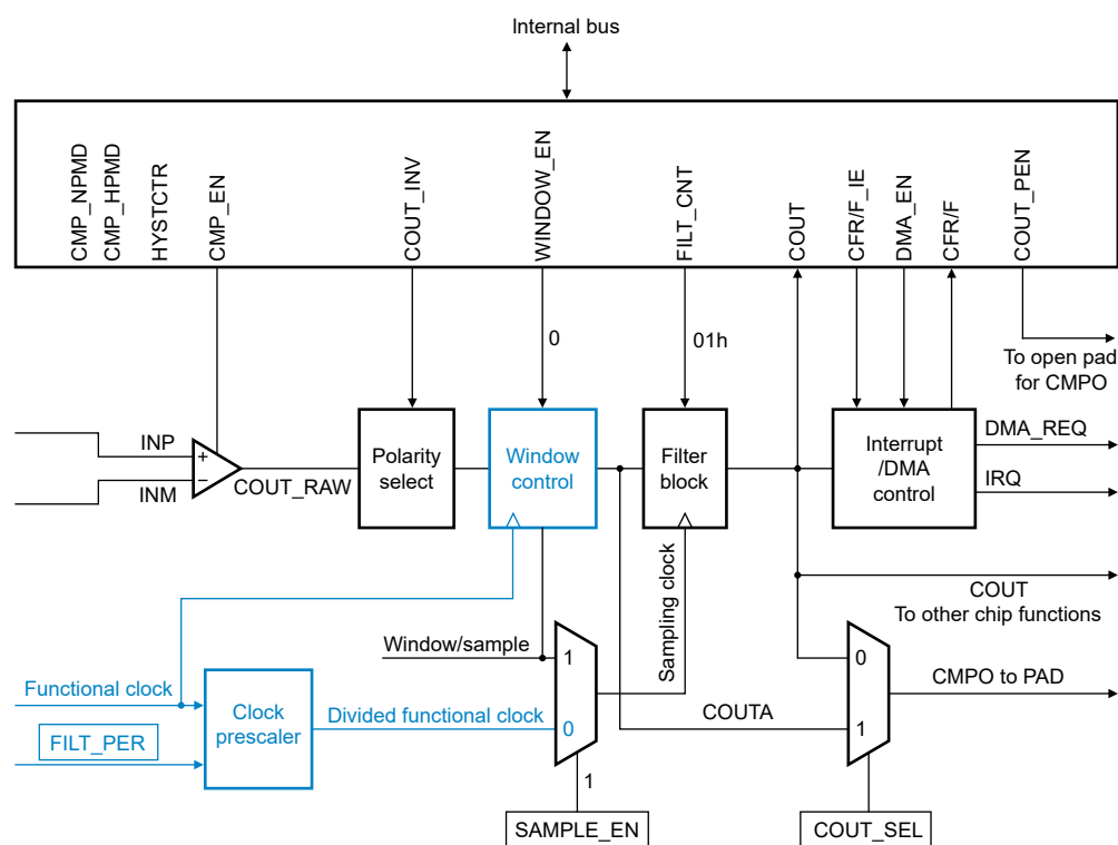
Figure 172. Sampled, non-filtered (#3A): sampling point externally driven
