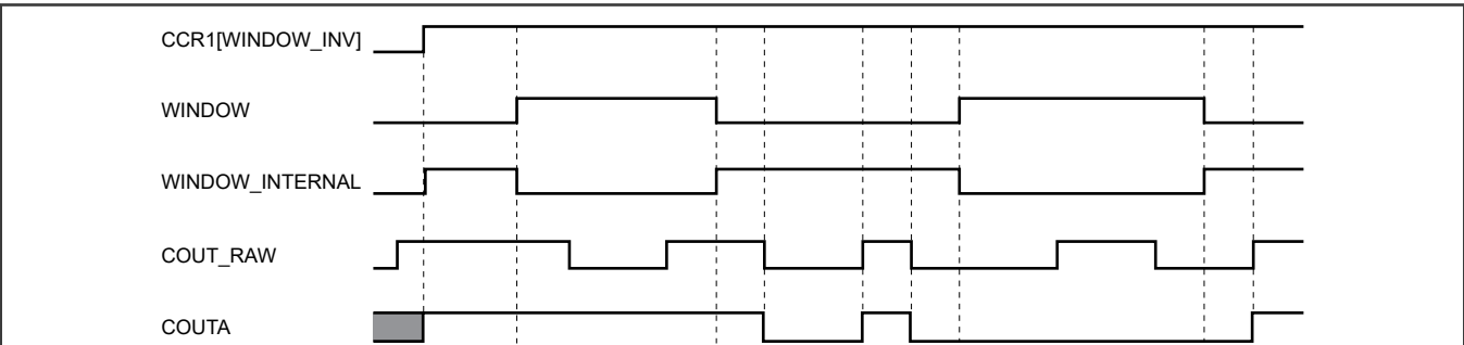
Figure 182. Windowed mode timing diagram with window signal inverted
