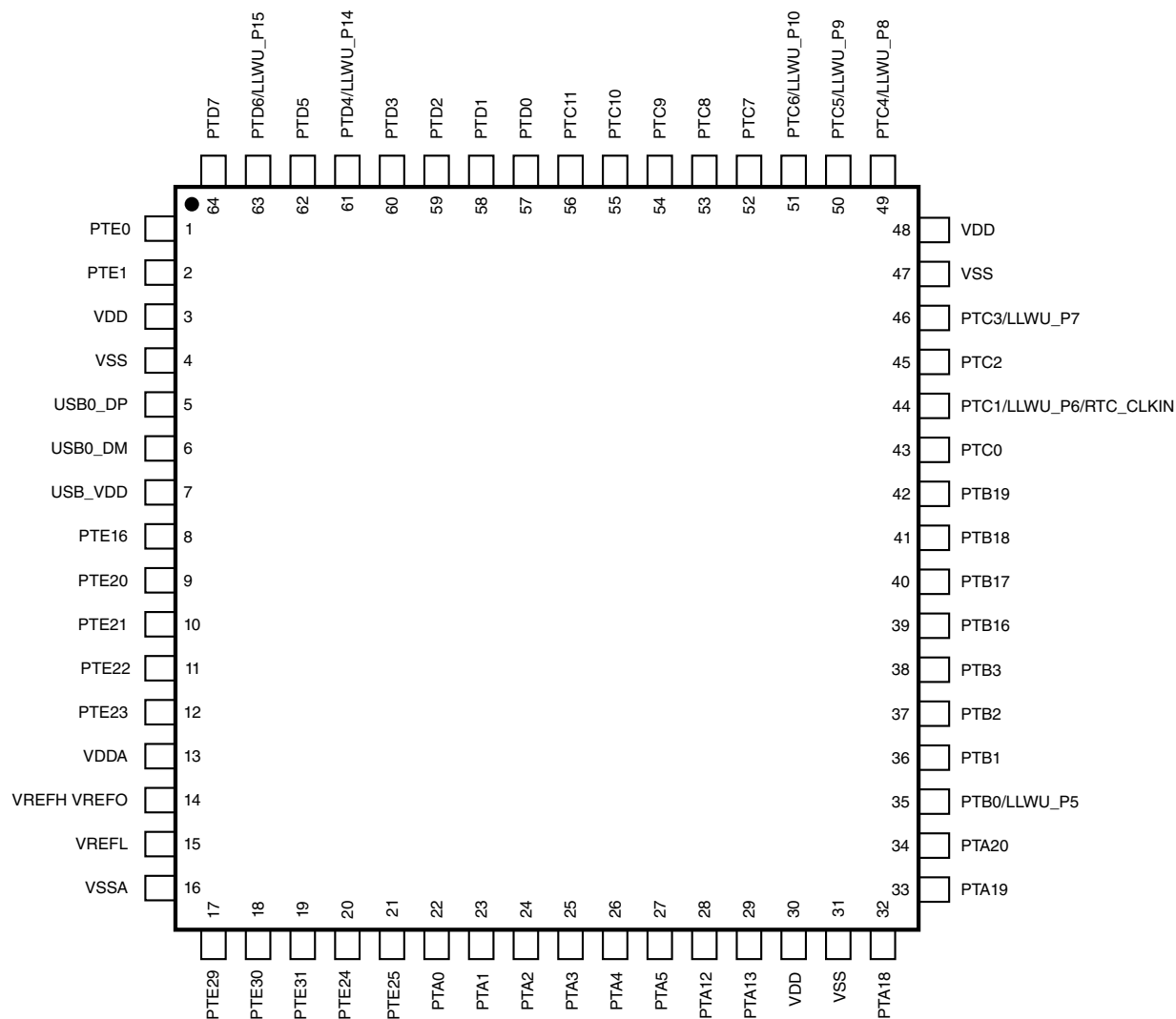
Figure 10-3. 64 LQFP Pinout diagram (top view)
