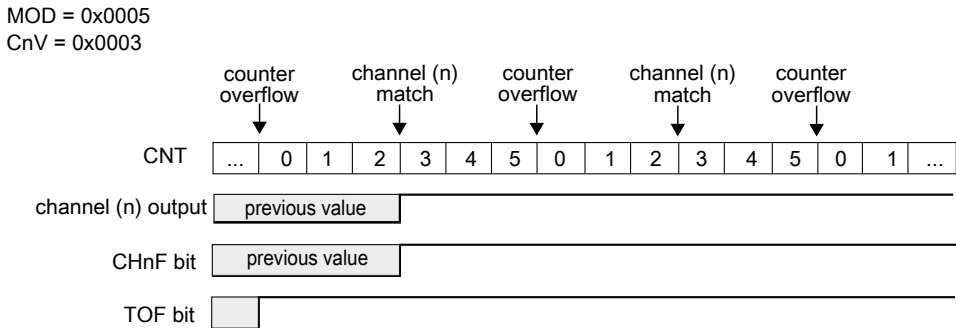
Figure 23-8. Example of the output compare mode when the match sets the channel output
