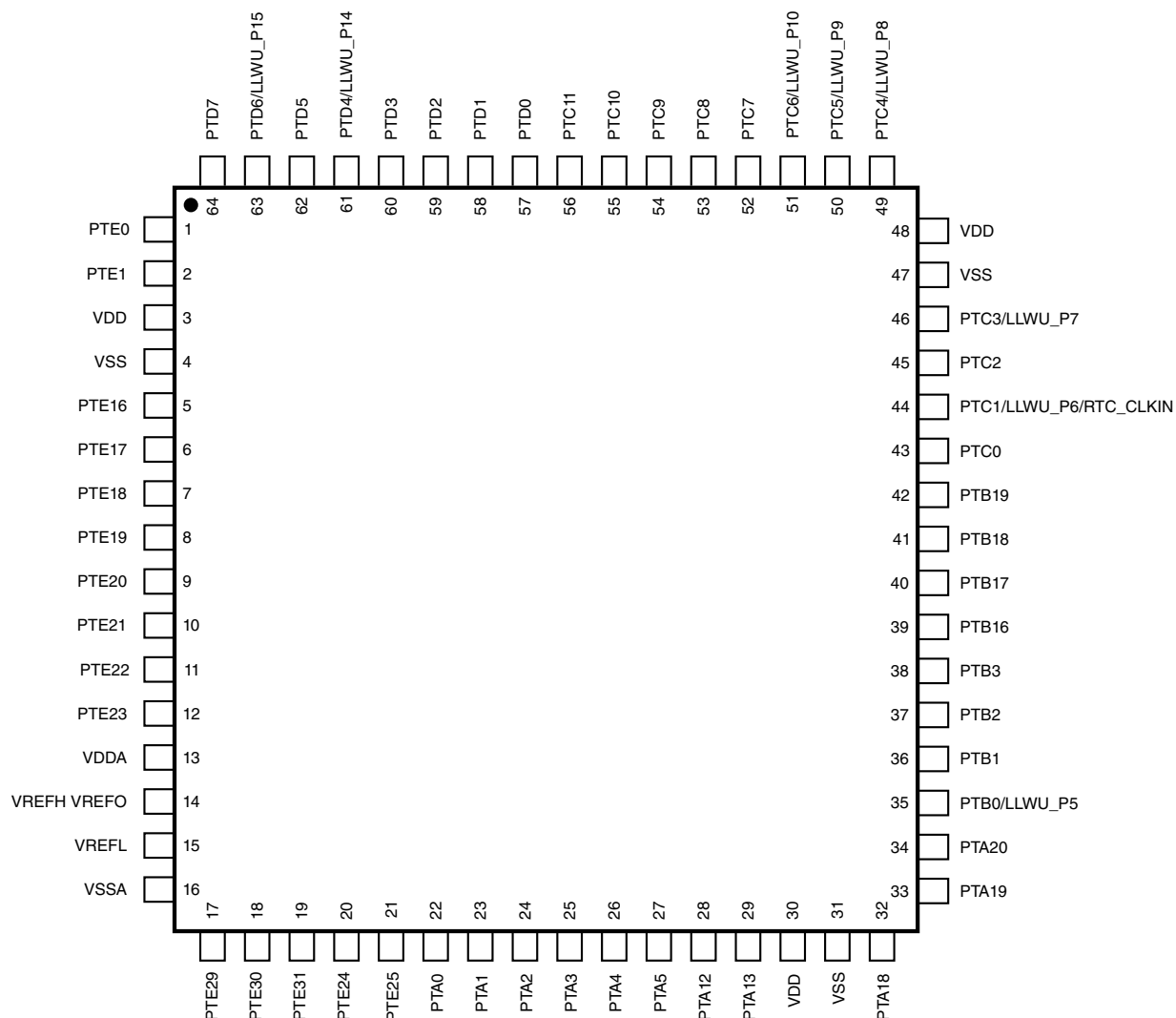
Figure 10-5. 64 LQFP Pinout diagram
