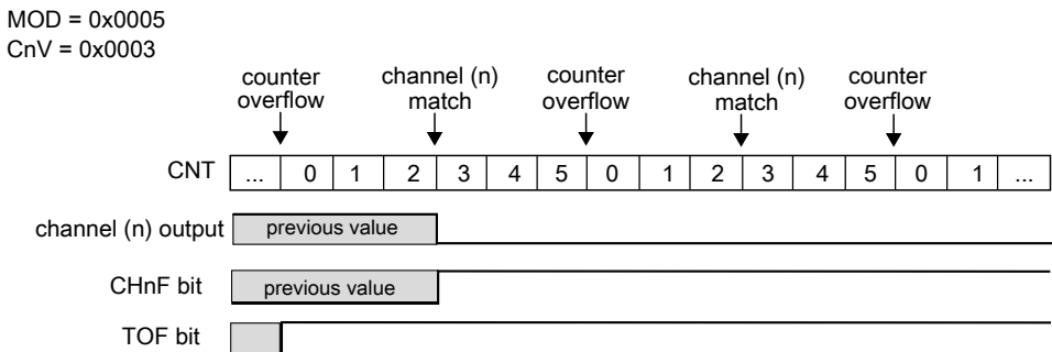
Figure 23-7. Example of the output compare mode when the match clears the channel output
