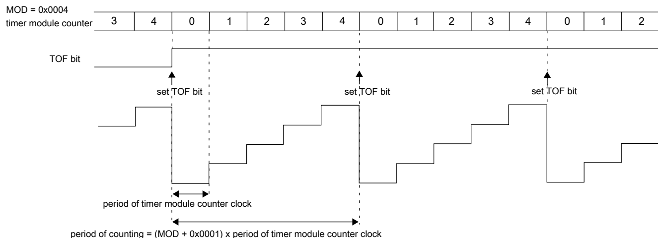
Figure 23-3. Example of TPM Up Counting
