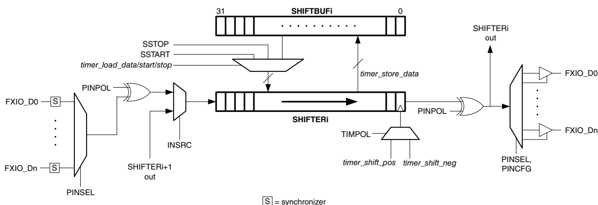
Figure 38-2. Shifter Microarchitecture
