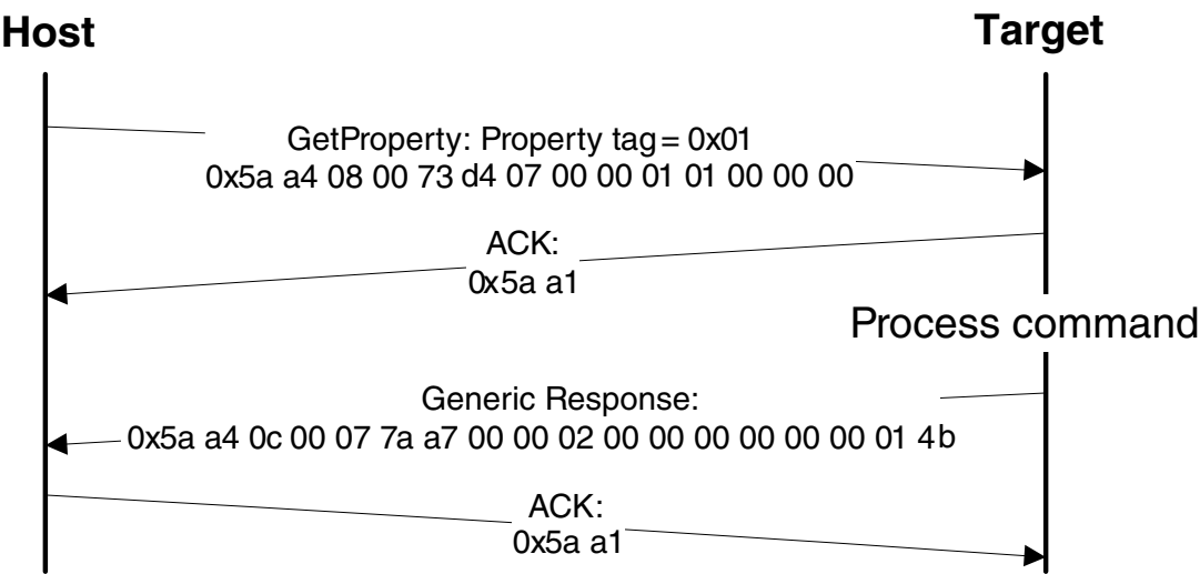
Figure 13-8. Protocol Sequence for GetProperty Command
