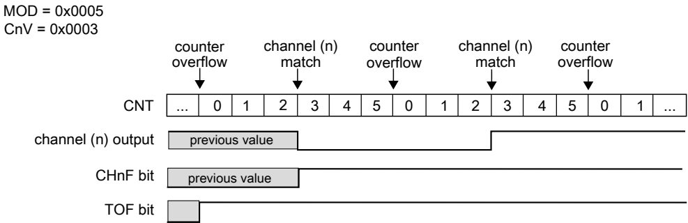
Figure 23-6. Example of the output compare mode when the match toggles the channel output
