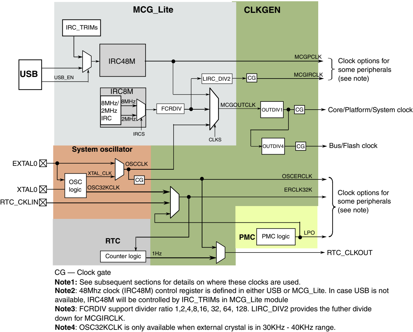
Figure 5-1. Clocking diagram
