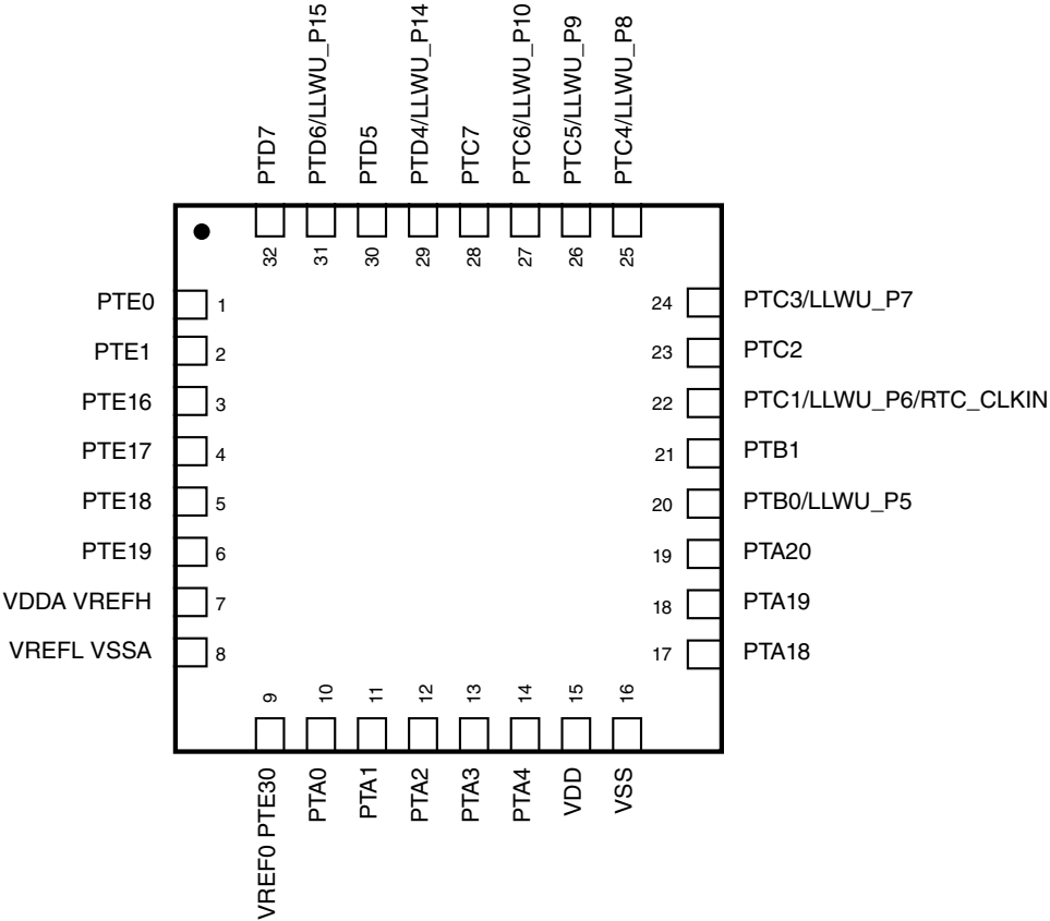
Figure 10-4. 32 QFN Pinout diagram
