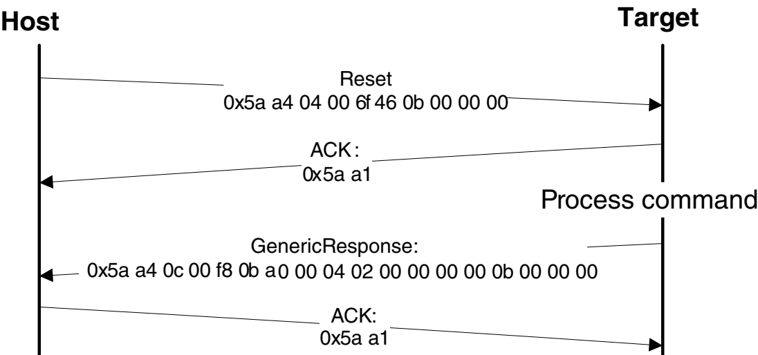
Figure 13-7. Protocol Sequence for Reset Command
