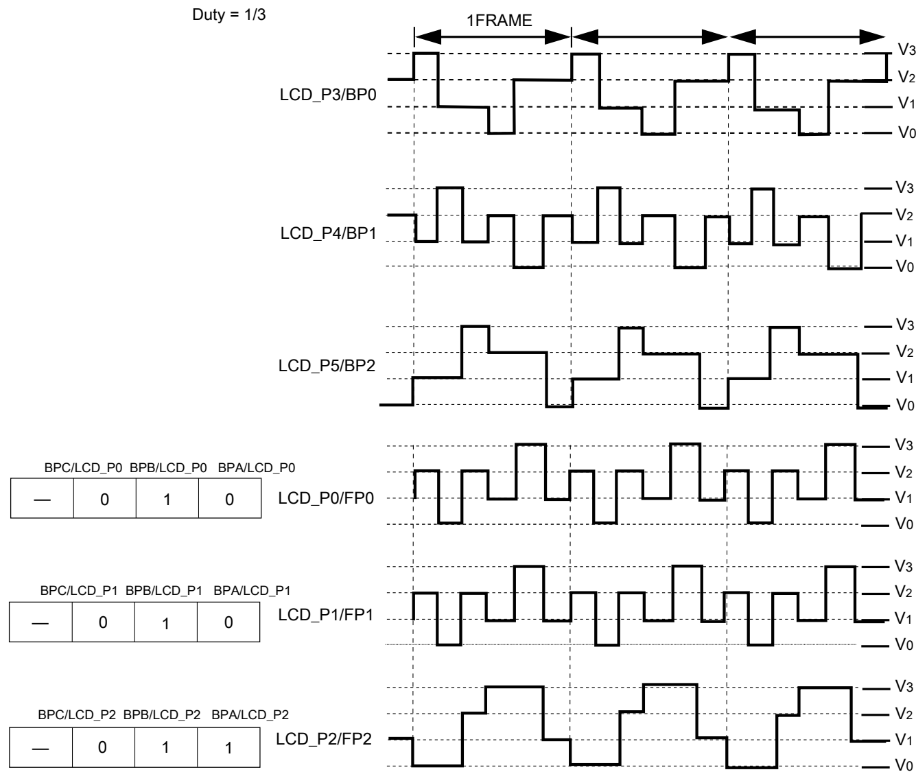
Figure 42-14. LCD waveforms
