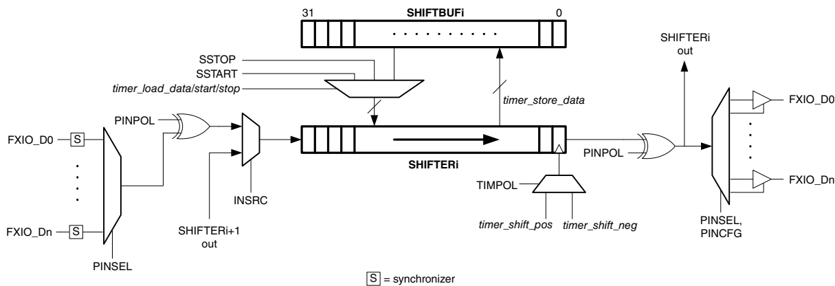
Figure 39-2. Shifter Microarchitecture
