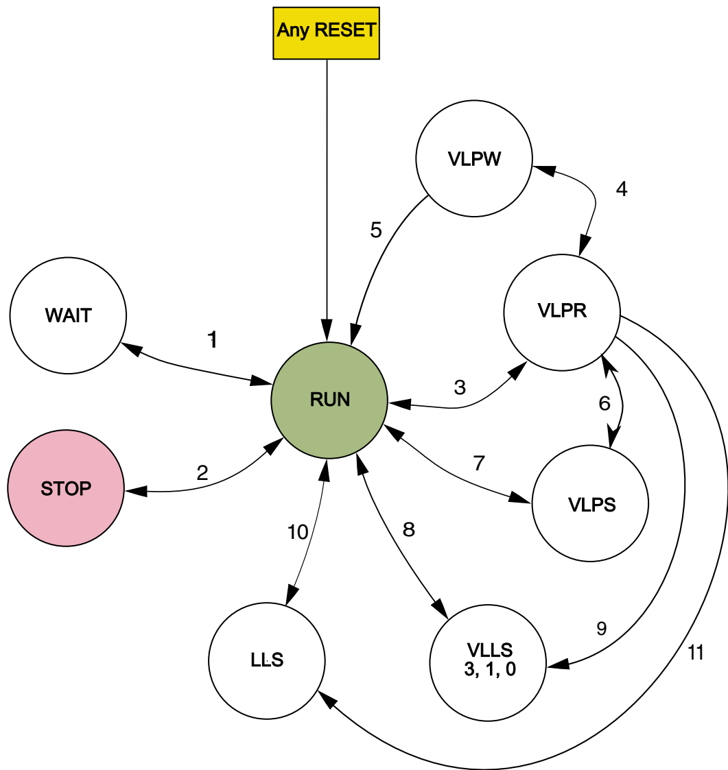
Figure 14-1. Power mode state diagram
