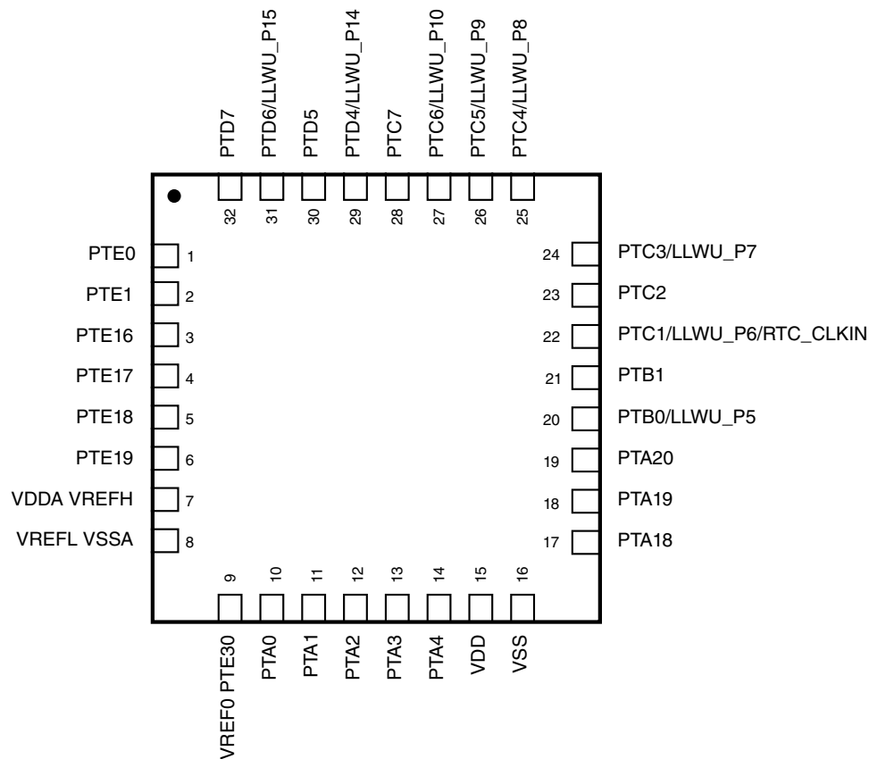
Figure 10-6. 32 QFN Pinout diagram
