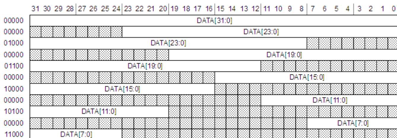
Figure 40-3. SAI first bit shifted, LSB first
