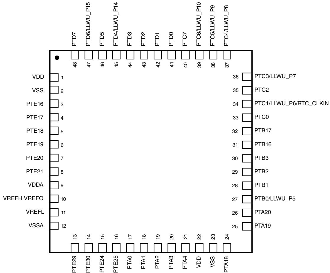
Figure 10-7. 48 QFN Pinout diagram
