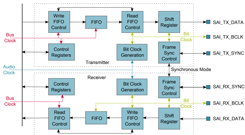
Figure 40-1. I²S/SAI block diagram
