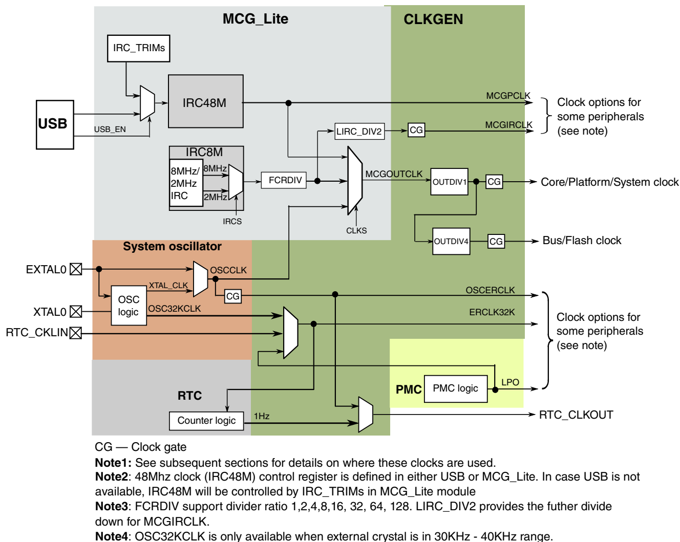
Figure 5-1. Clocking diagram
