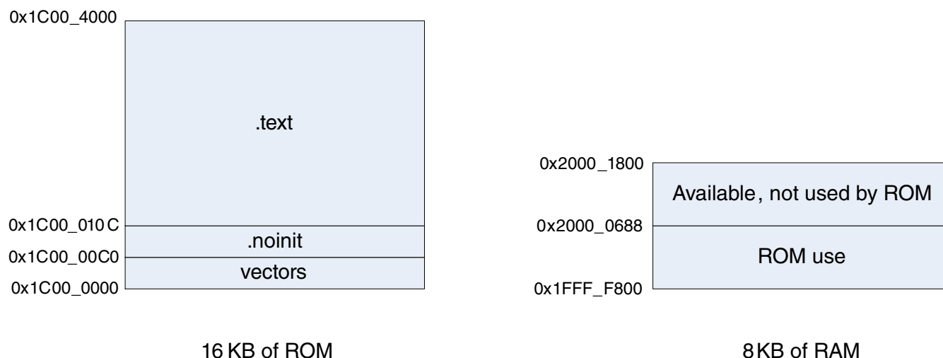
Figure 13-1. Bootloader ROM/RAM Memory Maps
