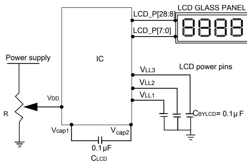
Figure 42-17. Power connections for contrast control
