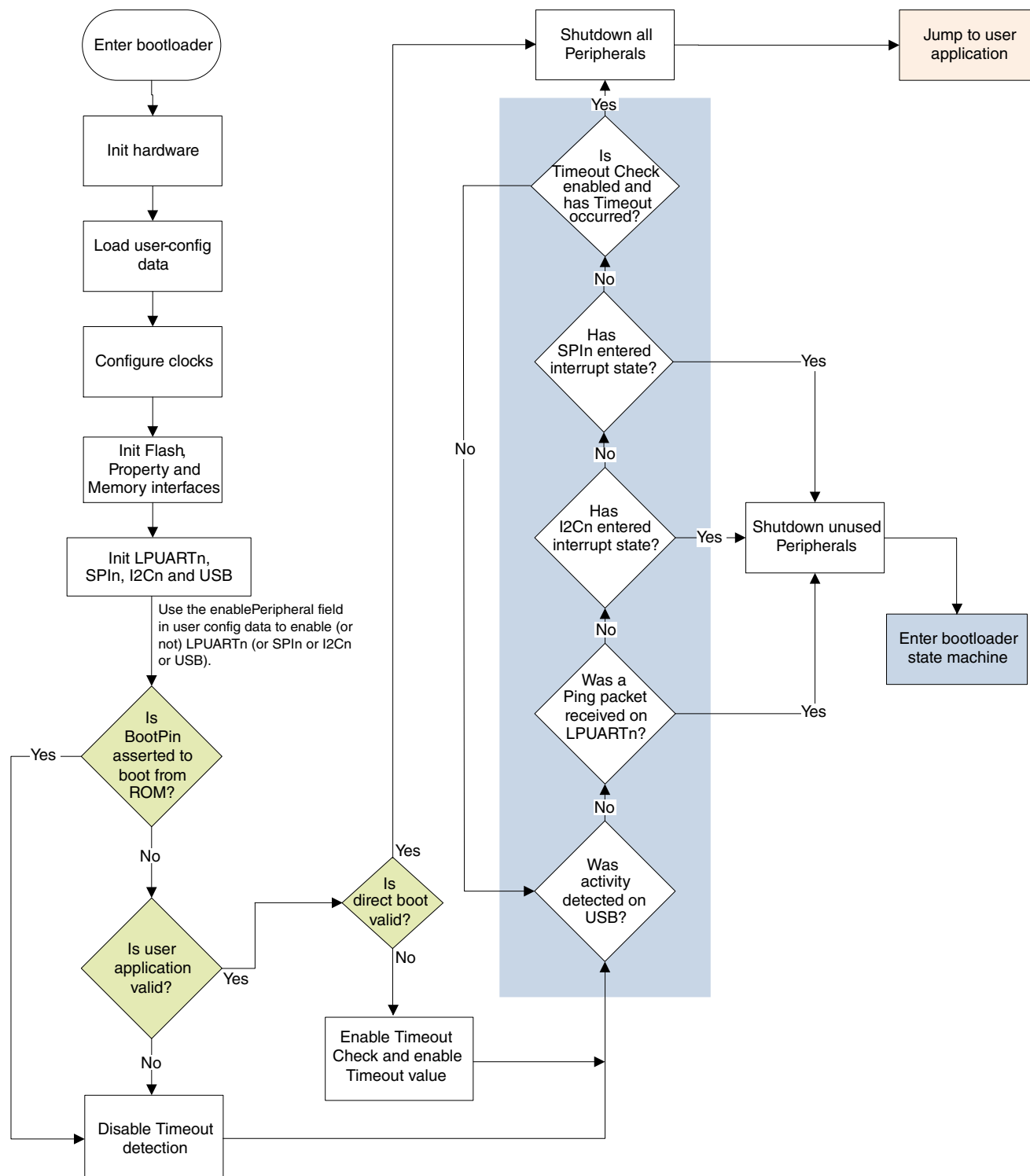
Figure 13-2. Bootloader Start-up Flowchart
