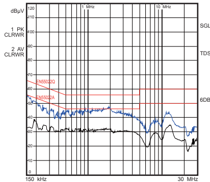
Conducted EMI
