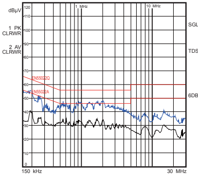
Conducted EMI
