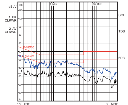
Conducted EMI
