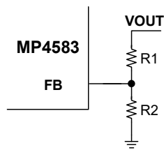
Figure 4: Feedback Network
