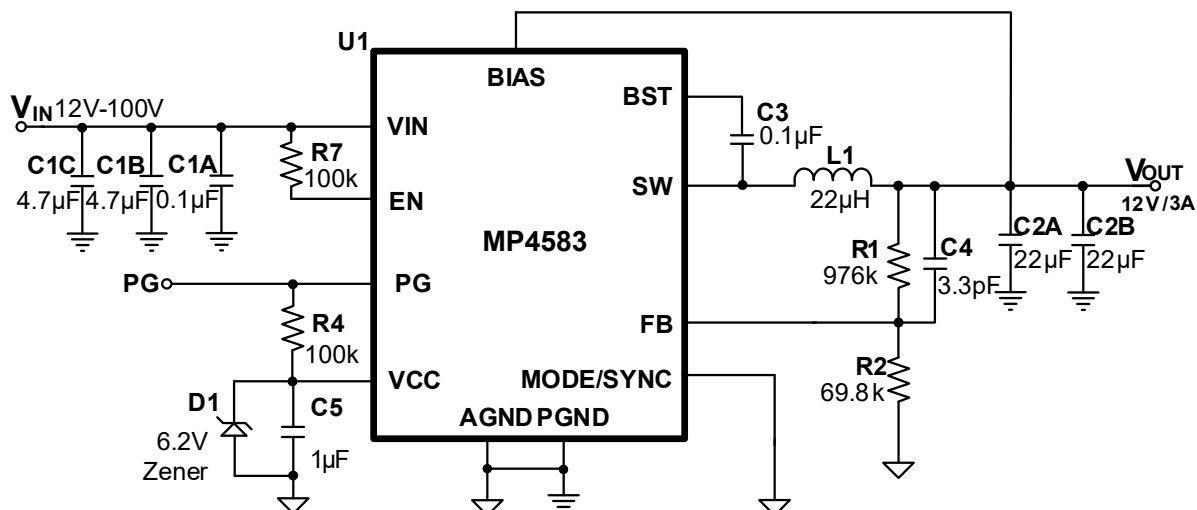
Figure 7: 12V Output Typical Application Circuit
