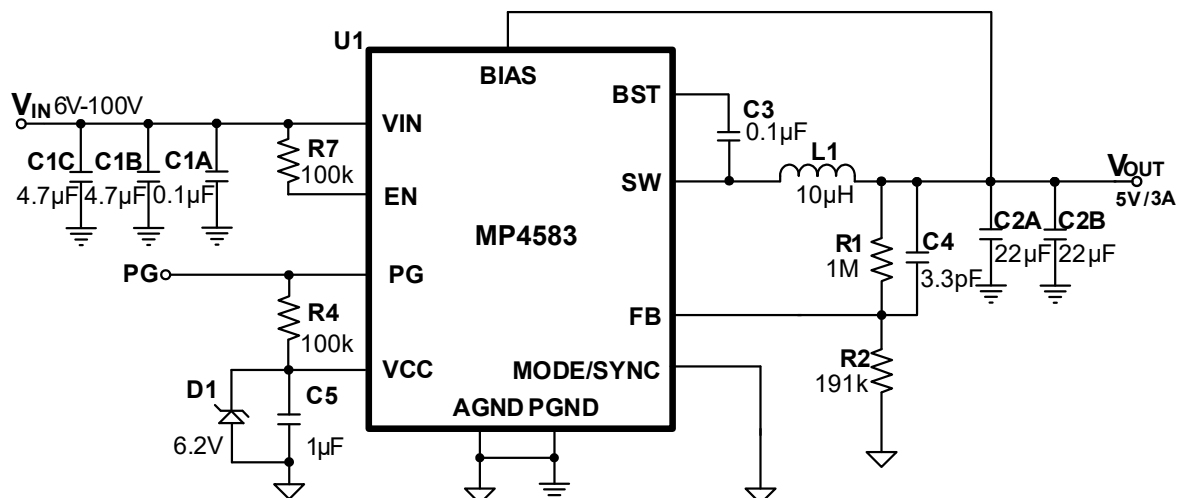
Figure 6: 5V Output Typical Application Circuit
