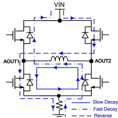
Figure 4: Reverse Operation
