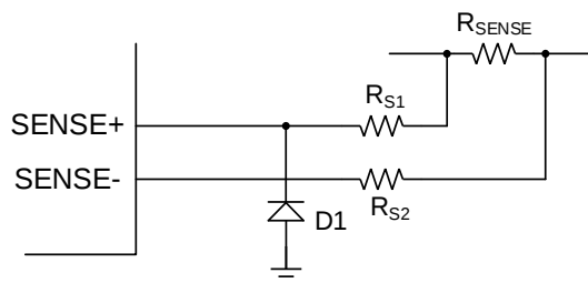
Figure 6: Negative Voltage Protection on SENSE+ and SENSE-
