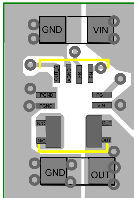
Figure 3: Top View of Layout Guide
