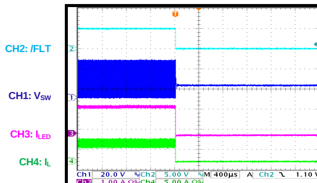
No Dimming LED+ to PGND short entry
