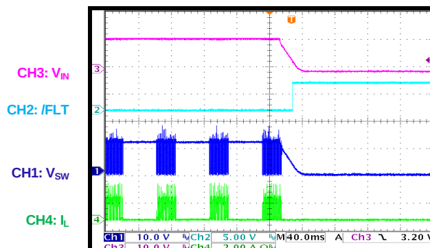
PWM Dimming LED+ to PGND short, shutdown
