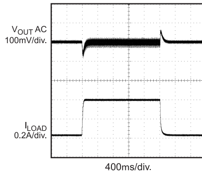
Transient Response
