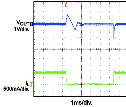
Load Transient Response I_{OUT}=0 \rightarrow 0.5A , 0.1A/\mu s
