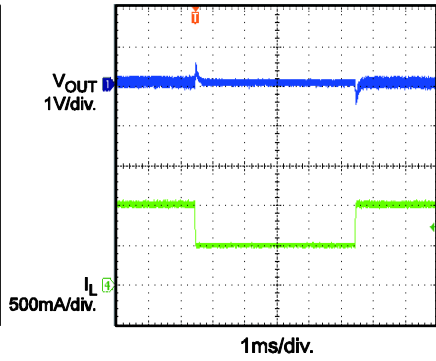
Load Transient Response I_{OUT}=0.5A \rightarrow 1A , 0.1A/\mu s
