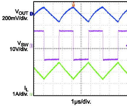
VOUT Ripple I_{OUT}=1A
