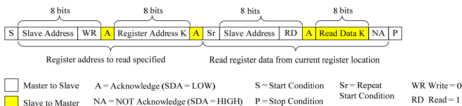
(b) I 2 C Read Example
