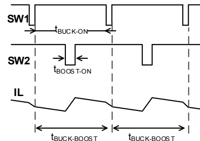
Figure 4: Buck-Boost Waveform
