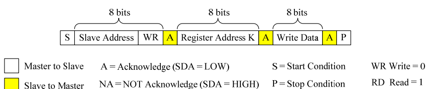
(a) I 2 C Write Example
