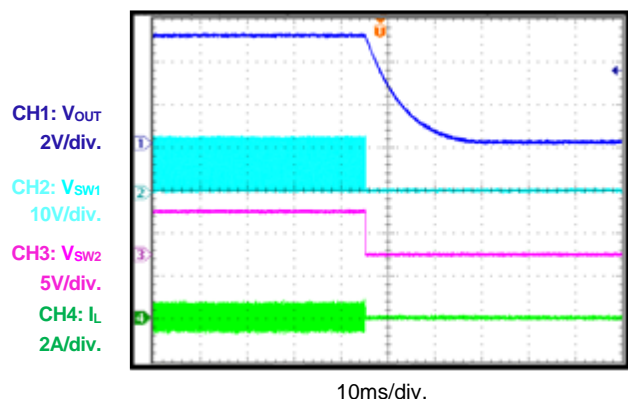
EN Pin Disable, Load = 10mA
