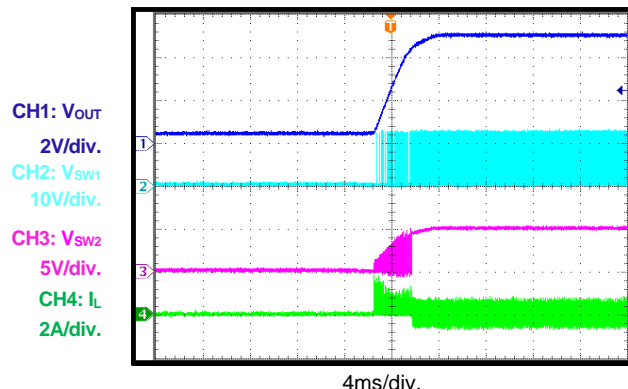
ENPWR Bit Enable through I 2 C Command, Load = 0A
