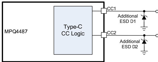
Figure 11: Recommended CC Pins ESD Enhancing
