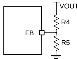
Figure 3 – Adjustable V_{OUT} by divider resistors can be chosen through below formula:
