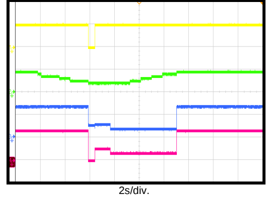
Mode Transition from 5V to 9V
