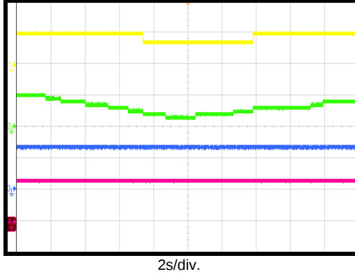
NTC Entry and Recovery for DCP Mode w/ QC
