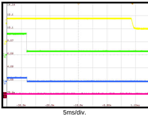
Mode Transition from 9V to 5V
