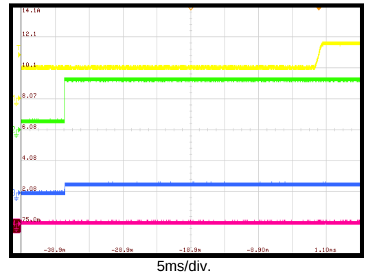
Mode Transition from 9V to 12V
