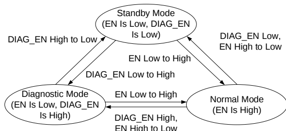
Figure 2: Operation Mode State Machine
