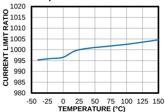
Current Limit Ratio vs. Temperature
