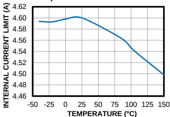
Internal Current Limit vs. Temperature
