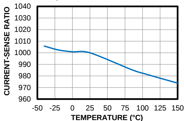
Current-Sense Ratio vs. Temperature
