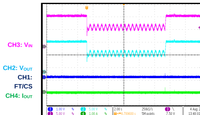
Cold Crank
