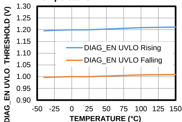
DIAG_EN UVLO Threshold vs. Temperature
