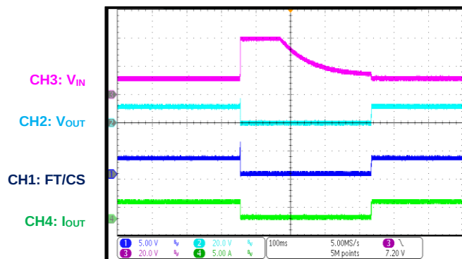
Load Dump
