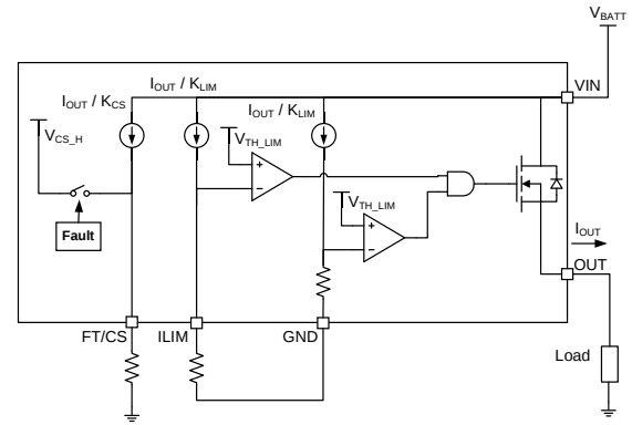
Figure 5: Current Sensing and Current Limit Functional Diagram
