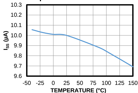
Soft-Start Current vs. Temperature
