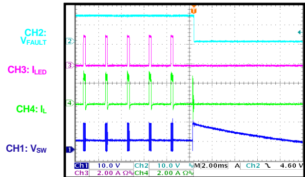
Two-Step Dimming LED open start-up
