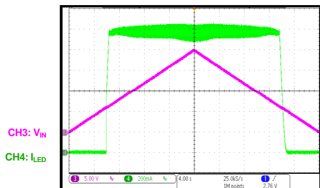
V_{IN} Slow Ramp Up and Down 2 LEDs ( V_{LED} = 6V ), I_{LED} = 1.2A , V_{IN} = 0V to 20V , 0.001V/ms
