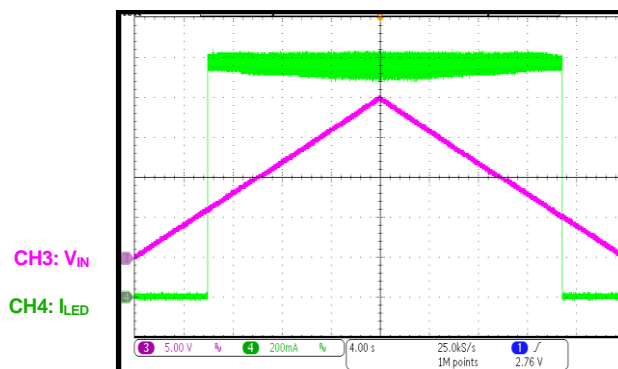
V_{IN} Slow Ramp Up and Down 1 LED ( V_{LED} = 3V ), I_{LED} = 1.2A , V_{IN} = 0V to 20V , 0.001V/ms
