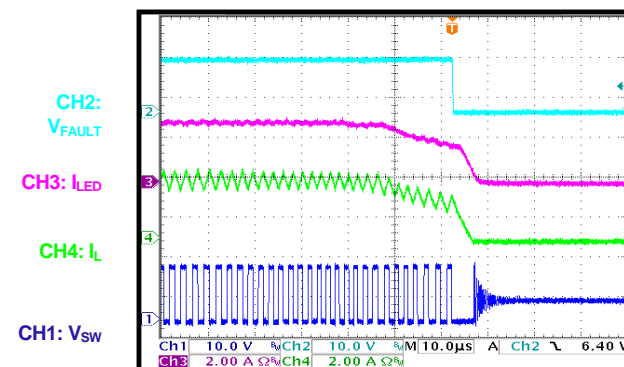
ISet Open after Start-Up
