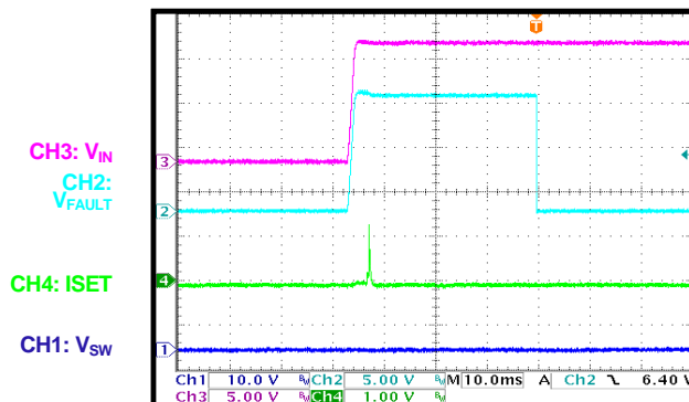
ISet Open before Start-Up
