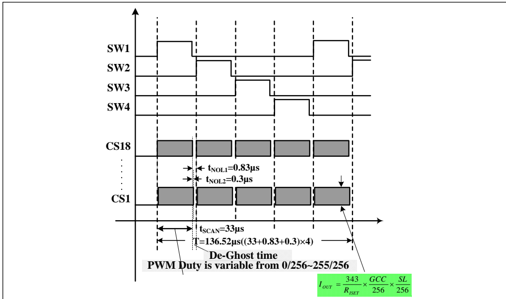
Figure 11 Scanning Timing
