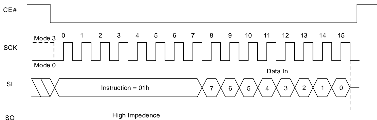
Figure 8.25 Write Status Register Sequence In SPI Mode
