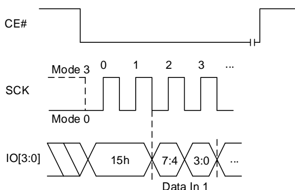
Figure 8.74 WRABR Sequence In QPI Mode
