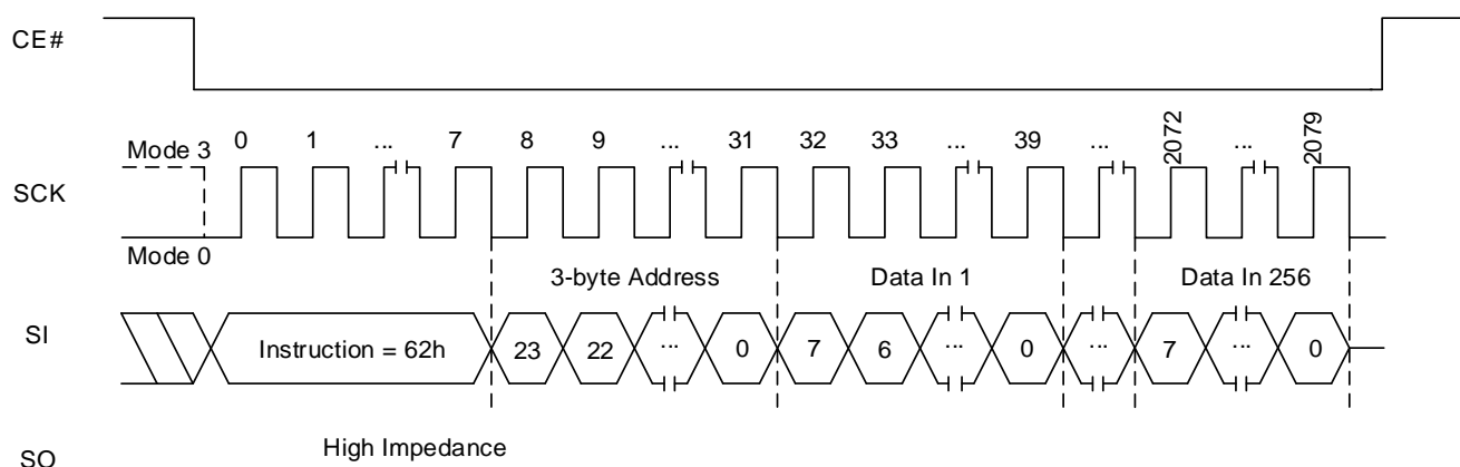
Figure 8.58 IRP (Information Row Program) Sequence
