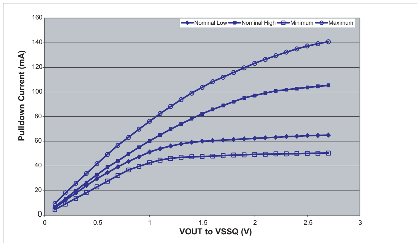
Pulldown characteristics for Full Strength Output Driver
