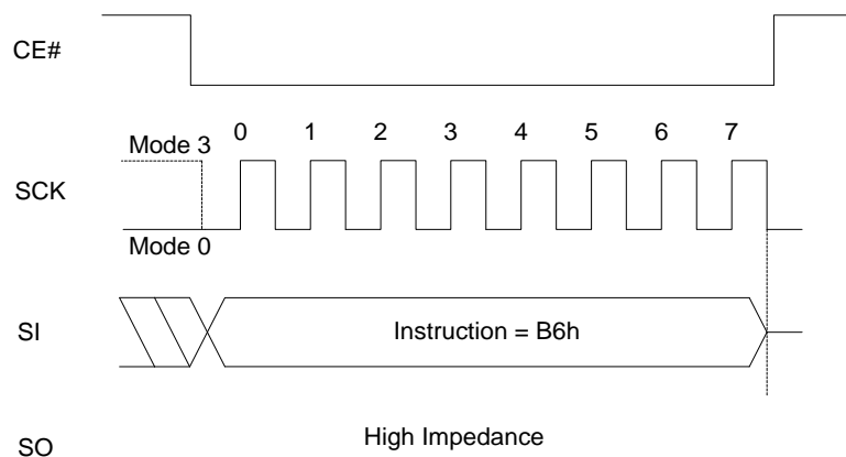
Figure 8.154 Clear ECC Register Sequence In SPI Mode
